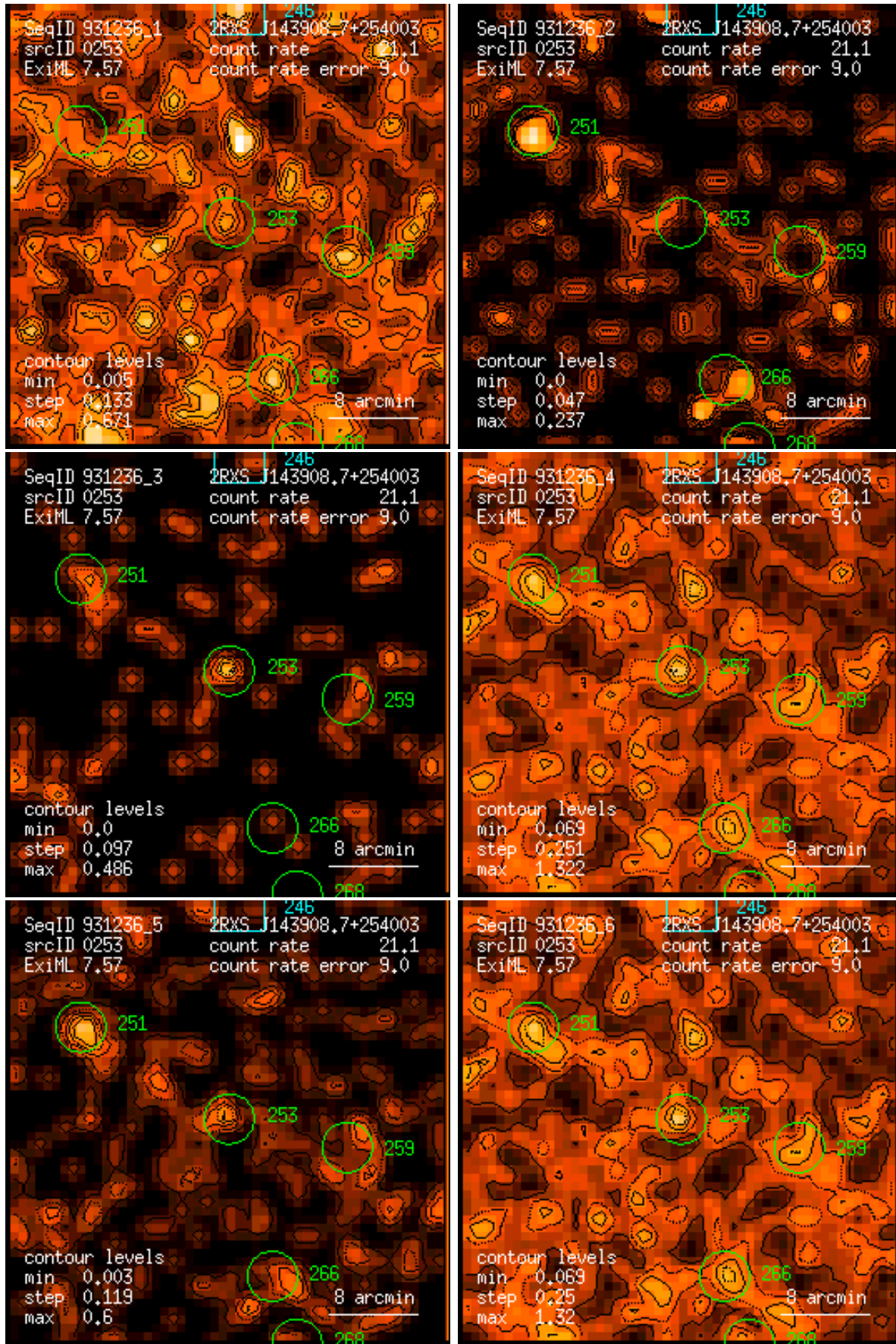
Figure 253: RASS 931236: detection 0253: band rate images, Gaussian filter: (1) PSPC channels 11 – 41, (2) 52 – 90, (3) 91 – 201, (4) 11 – 235, (5) 52 – 201, (6) 11 – 201. Broad band rates in counts/ks. Band rate contour levels in counts/ks/arcmin 2 .
