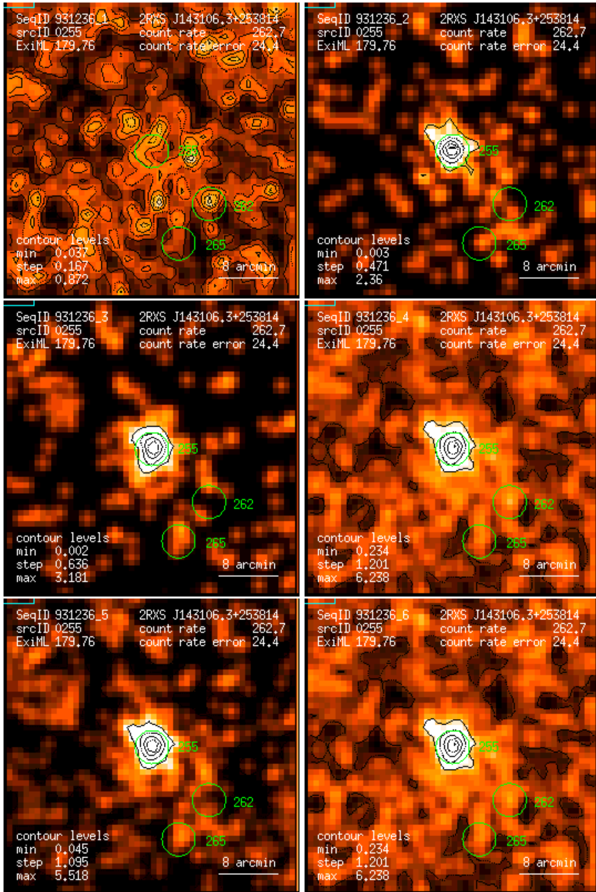
Figure 255: RASS 931236: detection 0255: band rate images, Gaussian filter: (1) PSPC channels 11 – 41, (2) 52 – 90, (3) 91 – 201, (4) 11 – 235, (5) 52 – 201, (6) 11 – 201. Broad band rates in counts/ks. Band rate contour levels in counts/ks/arcmin 2 .
