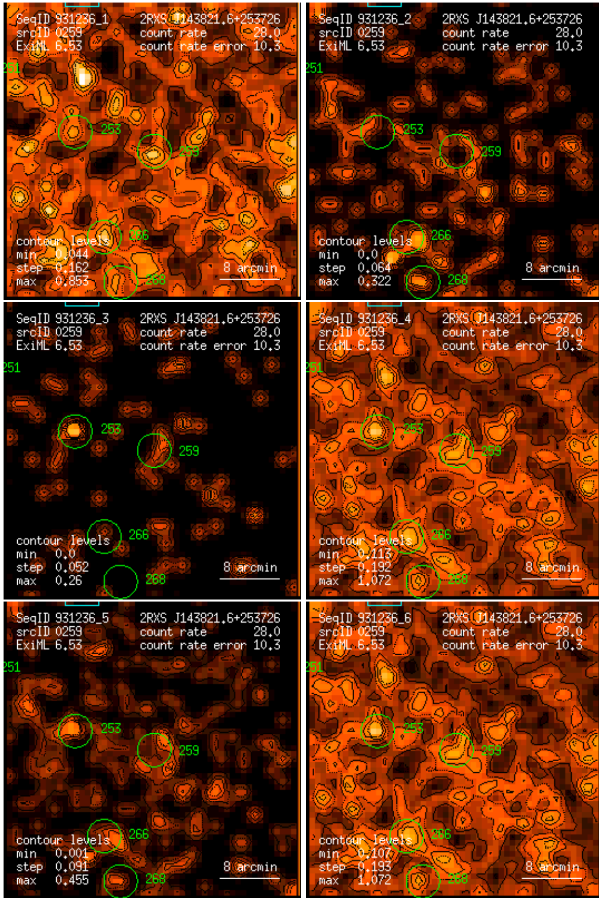
Figure 259: RASS 931236: detection 0259: band rate images, Gaussian filter: (1) PSPC channels 11 – 41, (2) 52 – 90, (3) 91 – 201, (4) 11 – 235, (5) 52 – 201, (6) 11 – 201. Broad band rates in counts/ks. Band rate contour levels in counts/ks/arcmin 2 .
