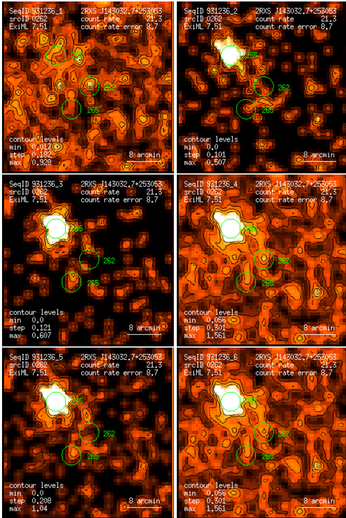
Figure 262: RASS 931236: detection 0262: band rate images, Gaussian filter: (1) PSPC channels 11 – 41, (2) 52 – 90, (3) 91 – 201, (4) 11 – 235, (5) 52 – 201, (6) 11 – 201. Broad band rates in counts/ks. Band rate contour levels in counts/ks/arcmin 2 .
