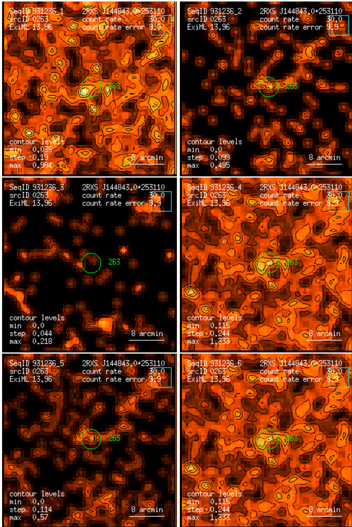
Figure 263: RASS 931236: detection 0263: band rate images, Gaussian filter: (1) PSPC channels 11 – 41, (2) 52 – 90, (3) 91 – 201, (4) 11 – 235, (5) 52 – 201, (6) 11 – 201. Broad band rates in counts/ks. Band rate contour levels in counts/ks/arcmin 2 .
