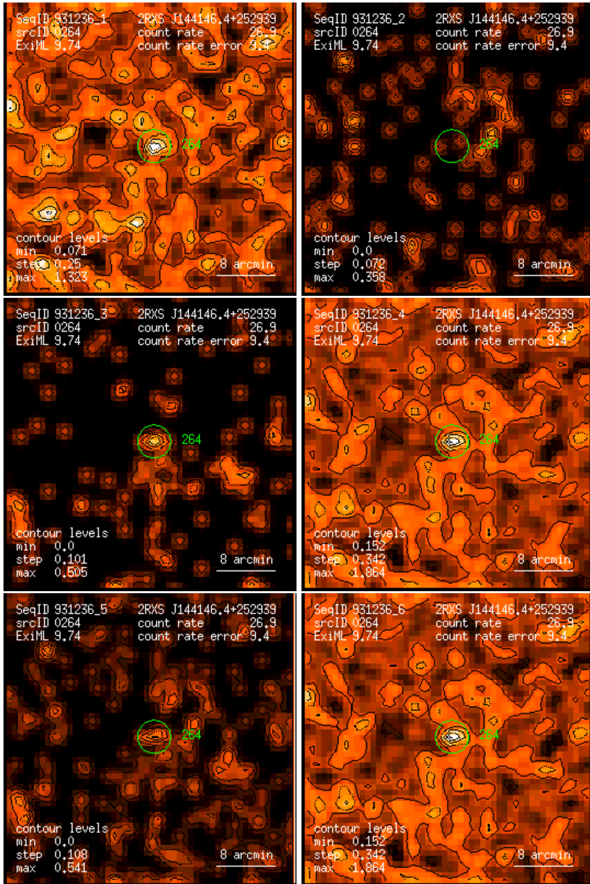
Figure 264: RASS 931236: detection 0264: band rate images, Gaussian filter: (1) PSPC channels 11 – 41, (2) 52 – 90, (3) 91 – 201, (4) 11 – 235, (5) 52 – 201, (6) 11 – 201. Broad band rates in counts/ks. Band rate contour levels in counts/ks/arcmin 2 .
