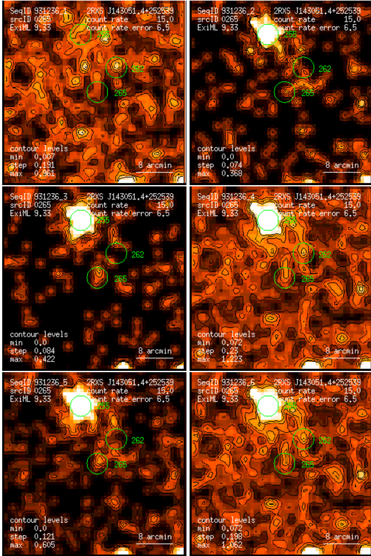
Figure 265: RASS 931236: detection 0265: band rate images, Gaussian filter: (1) PSPC channels 11 – 41, (2) 52 – 90, (3) 91 – 201, (4) 11 – 235, (5) 52 – 201, (6) 11 – 201. Broad band rates in counts/ks. Band rate contour levels in counts/ks/arcmin 2 .
