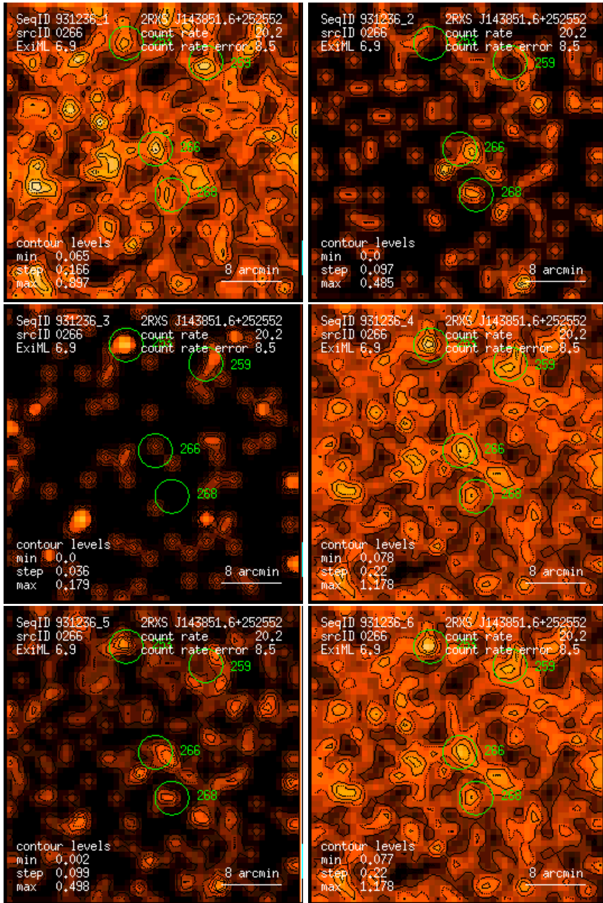
Figure 266: RASS 931236: detection 0266: band rate images, Gaussian filter: (1) PSPC channels 11 – 41, (2) 52 – 90, (3) 91 – 201, (4) 11 – 235, (5) 52 – 201, (6) 11 – 201. Broad band rates in counts/ks. Band rate contour levels in counts/ks/arcmin 2 .
