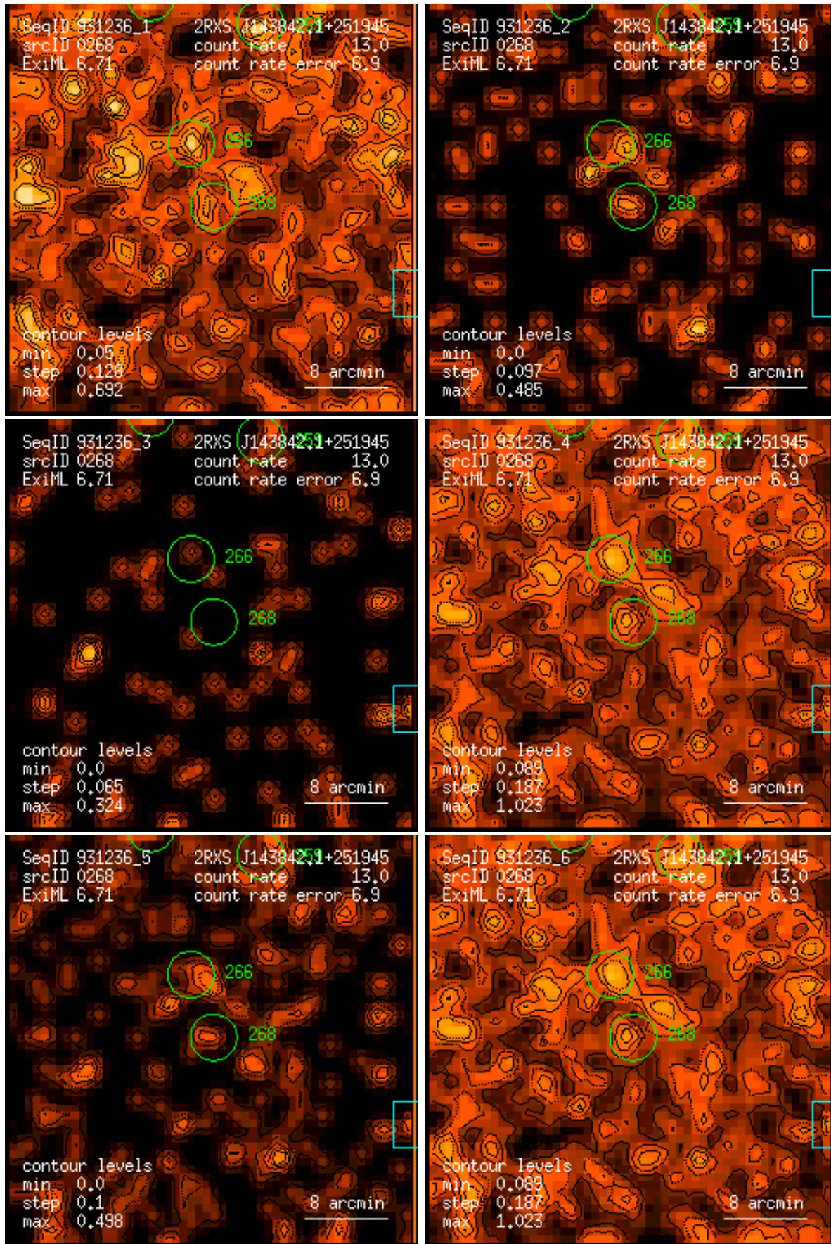
Figure 268: RASS 931236: detection 0268: band rate images, Gaussian filter: (1) PSPC channels 11 – 41, (2) 52 – 90, (3) 91 – 201, (4) 11 – 235, (5) 52 – 201, (6) 11 – 201. Broad band rates in counts/ks. Band rate contour levels in counts/ks/arcmin 2 .
