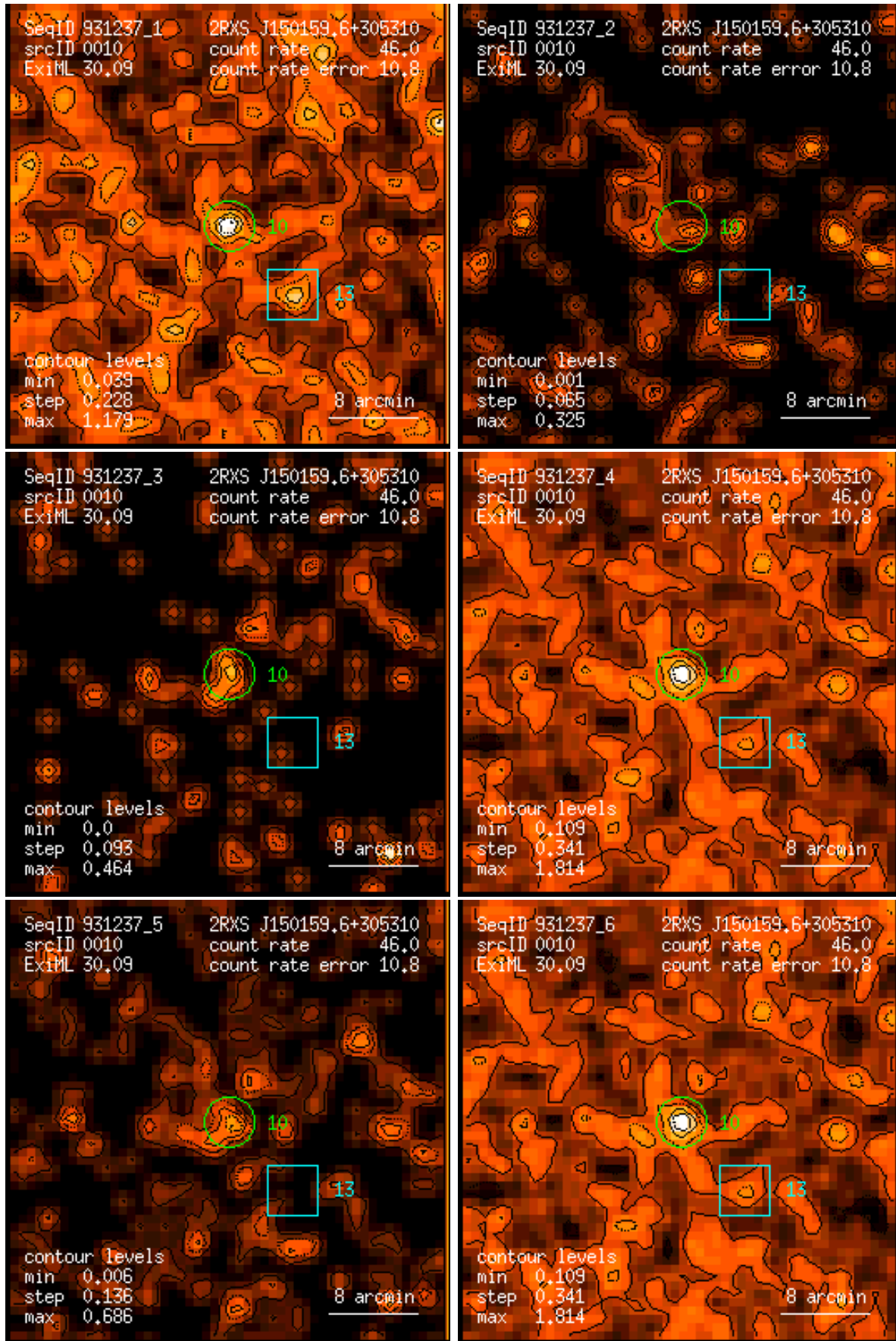
Figure 10: RASS 931237: detection 0010: band rate images, Gaussian filter: (1) PSPC channels 11 – 41, (2) 52 – 90, (3) 91 – 201, (4) 11 – 235, (5) 52 – 201, (6) 11 – 201. Broad band rates in counts/ks. Band rate contour levels in counts/ks/arcmin 2 .
