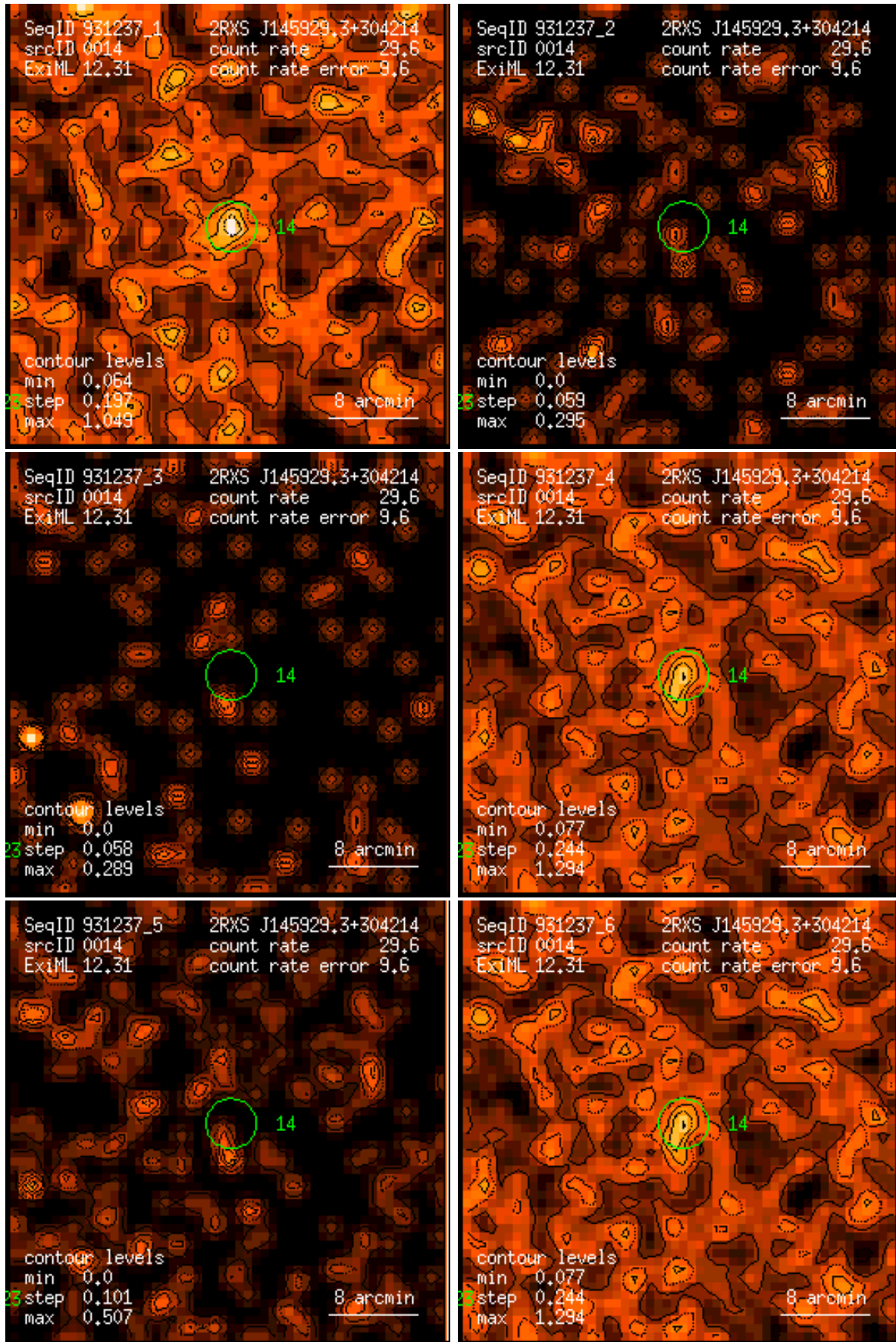
Figure 14: RASS 931237: detection 0014: band rate images, Gaussian filter: (1) PSPC channels 11 – 41, (2) 52 – 90, (3) 91 – 201, (4) 11 – 235, (5) 52 – 201, (6) 11 – 201. Broad band rates in counts/ks. Band rate contour levels in counts/ks/arcmin 2 .
