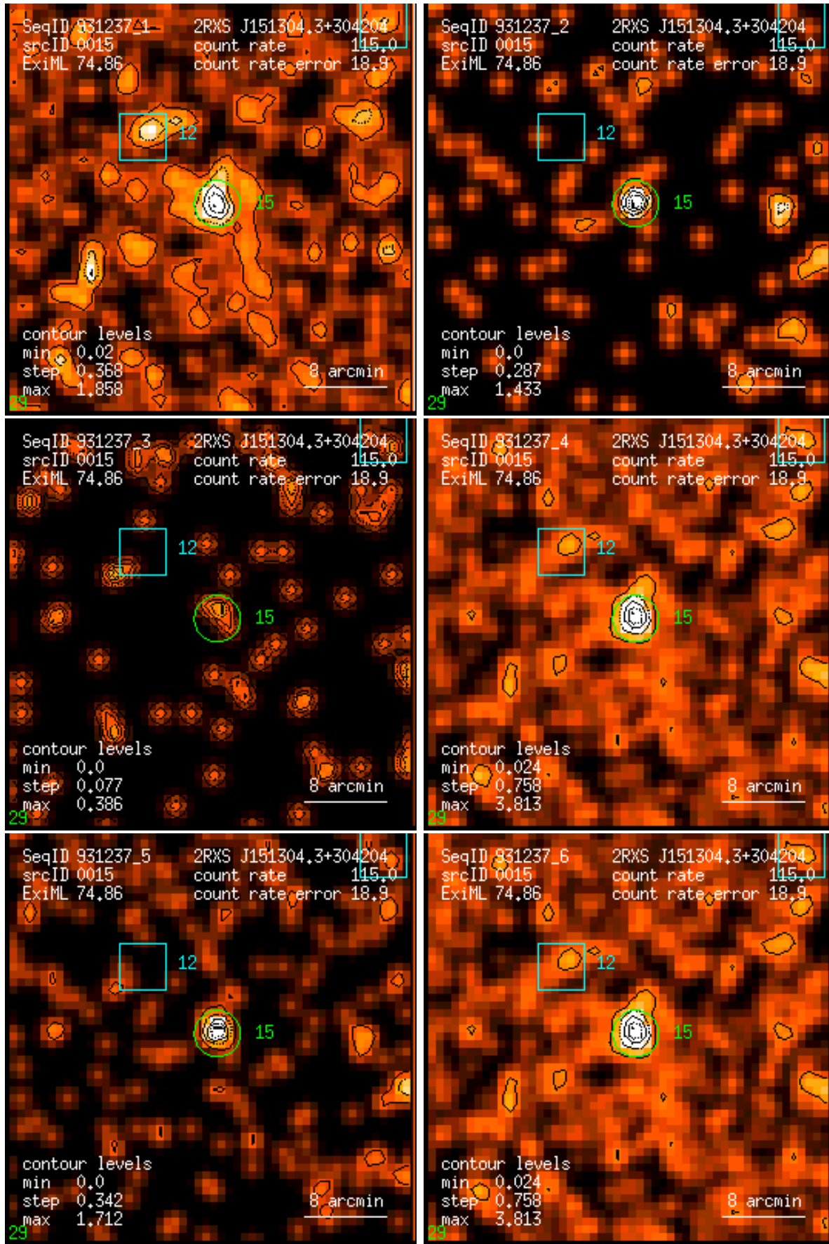
Figure 15: RASS 931237: detection 0015: band rate images, Gaussian filter: (1) PSPC channels 11 – 41, (2) 52 – 90, (3) 91 – 201, (4) 11 – 235, (5) 52 – 201, (6) 11 – 201. Broad band rates in counts/ks. Band rate contour levels in counts/ks/arcmin 2 .
