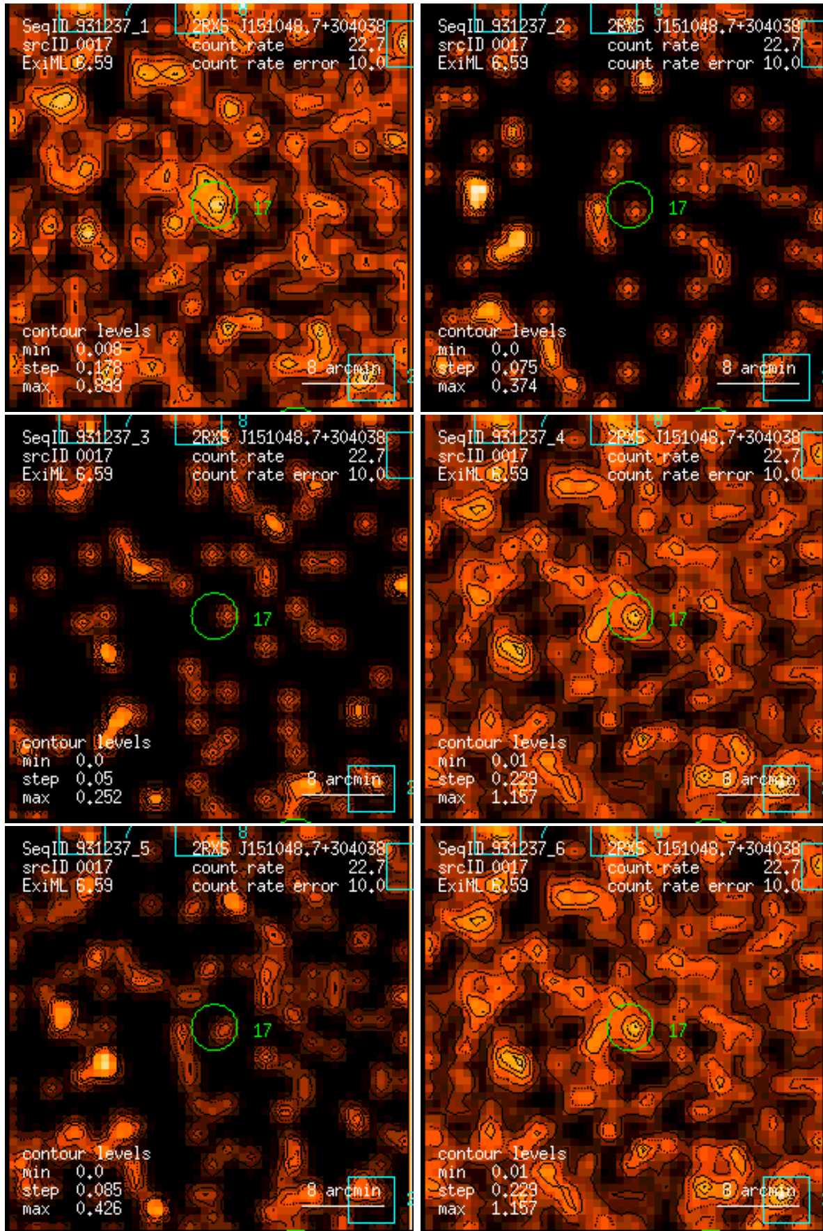
Figure 17: RASS 931237: detection 0017: band rate images, Gaussian filter: (1) PSPC channels 11 – 41, (2) 52 – 90, (3) 91 – 201, (4) 11 – 235, (5) 52 – 201, (6) 11 – 201. Broad band rates in counts/ks. Band rate contour levels in counts/ks/arcmin 2 .
