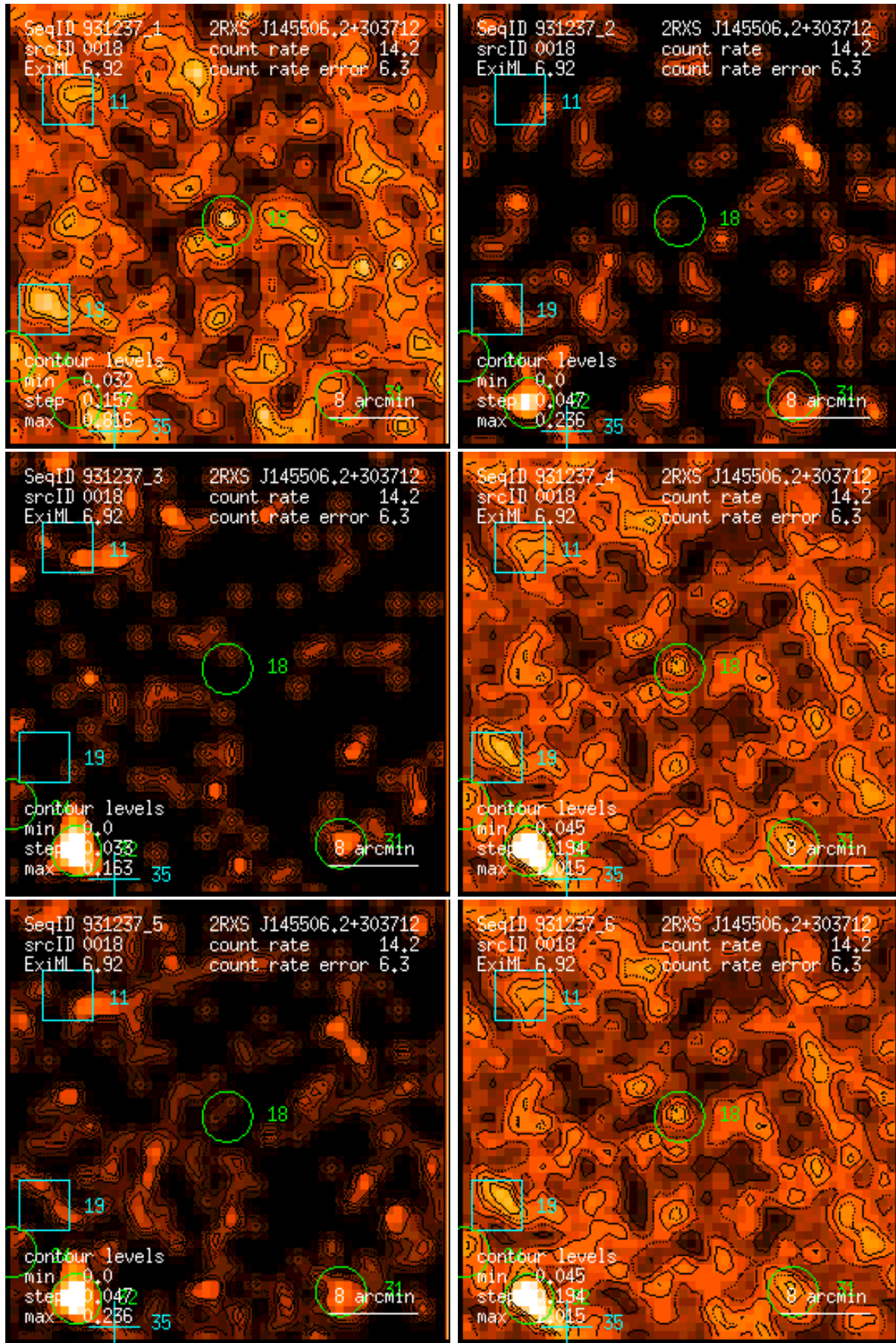
Figure 18: RASS 931237: detection 0018: band rate images, Gaussian filter: (1) PSPC channels 11 – 41, (2) 52 – 90, (3) 91 – 201, (4) 11 – 235, (5) 52 – 201, (6) 11 – 201. Broad band rates in counts/ks. Band rate contour levels in counts/ks/arcmin 2 .
