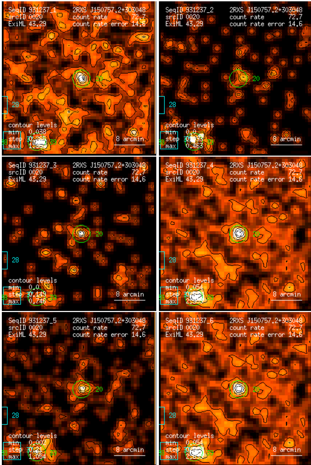
Figure 20: RASS 931237: detection 0020: band rate images, Gaussian filter: (1) PSPC channels 11 – 41, (2) 52 – 90, (3) 91 – 201, (4) 11 – 235, (5) 52 – 201, (6) 11 – 201. Broad band rates in counts/ks. Band rate contour levels in counts/ks/arcmin 2 .
