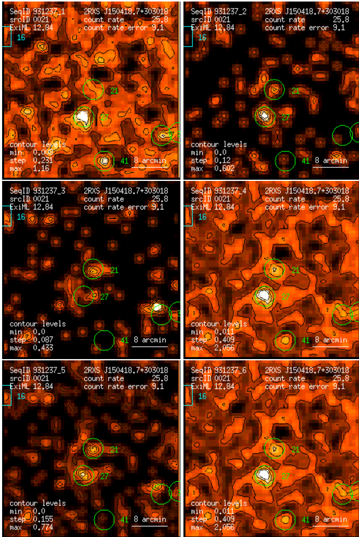
Figure 21: RASS 931237: detection 0021: band rate images, Gaussian filter: (1) PSPC channels 11 – 41, (2) 52 – 90, (3) 91 – 201, (4) 11 – 235, (5) 52 – 201, (6) 11 – 201. Broad band rates in counts/ks. Band rate contour levels in counts/ks/arcmin 2 .
