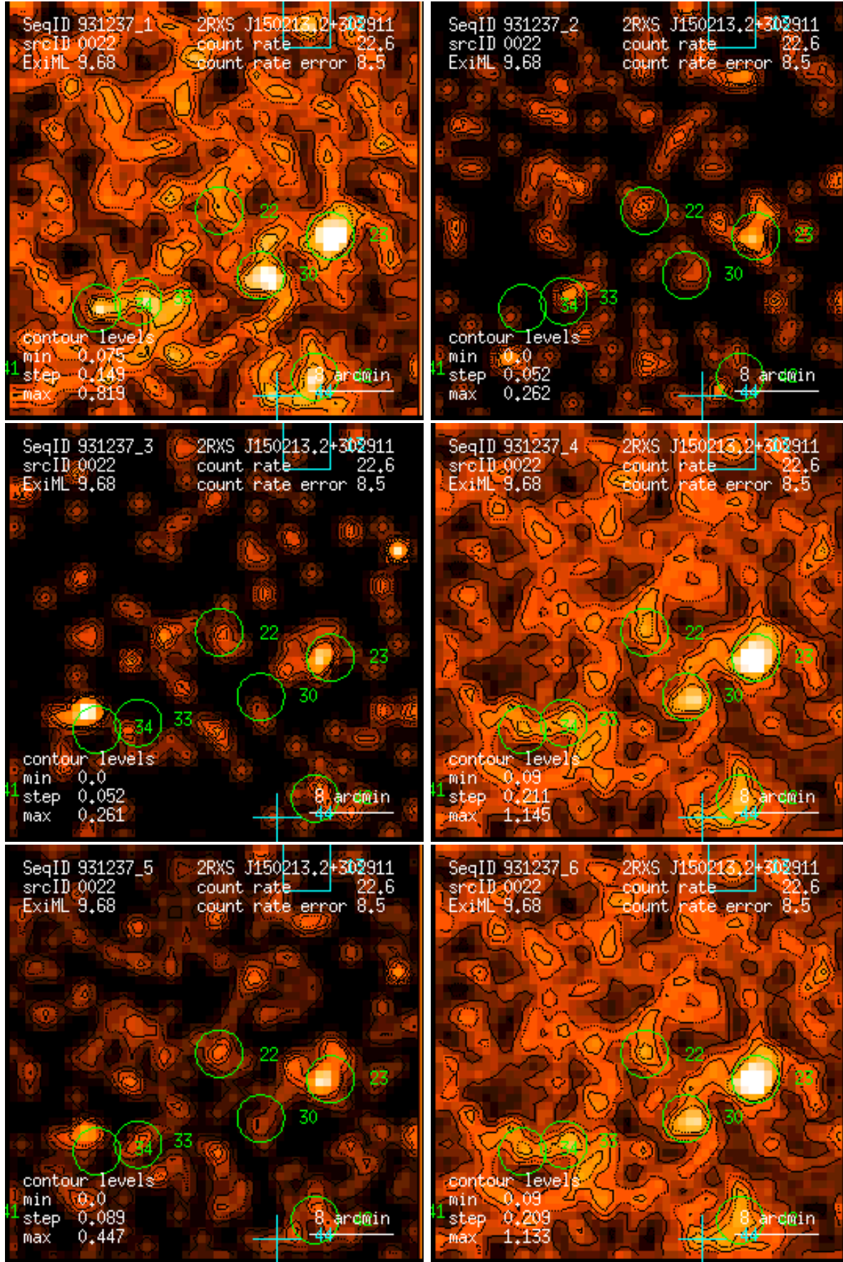
Figure 22: RASS 931237: detection 0022: band rate images, Gaussian filter: (1) PSPC channels 11 – 41, (2) 52 – 90, (3) 91 – 201, (4) 11 – 235, (5) 52 – 201, (6) 11 – 201. Broad band rates in counts/ks. Band rate contour levels in counts/ks/arcmin 2 .
