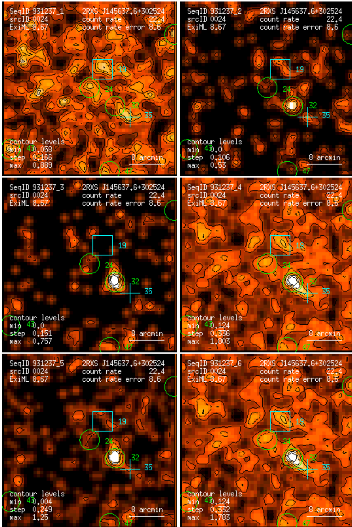
Figure 24: RASS 931237: detection 0024: band rate images, Gaussian filter: (1) PSPC channels 11 – 41, (2) 52 – 90, (3) 91 – 201, (4) 11 – 235, (5) 52 – 201, (6) 11 – 201. Broad band rates in counts/ks. Band rate contour levels in counts/ks/arcmin 2 .
