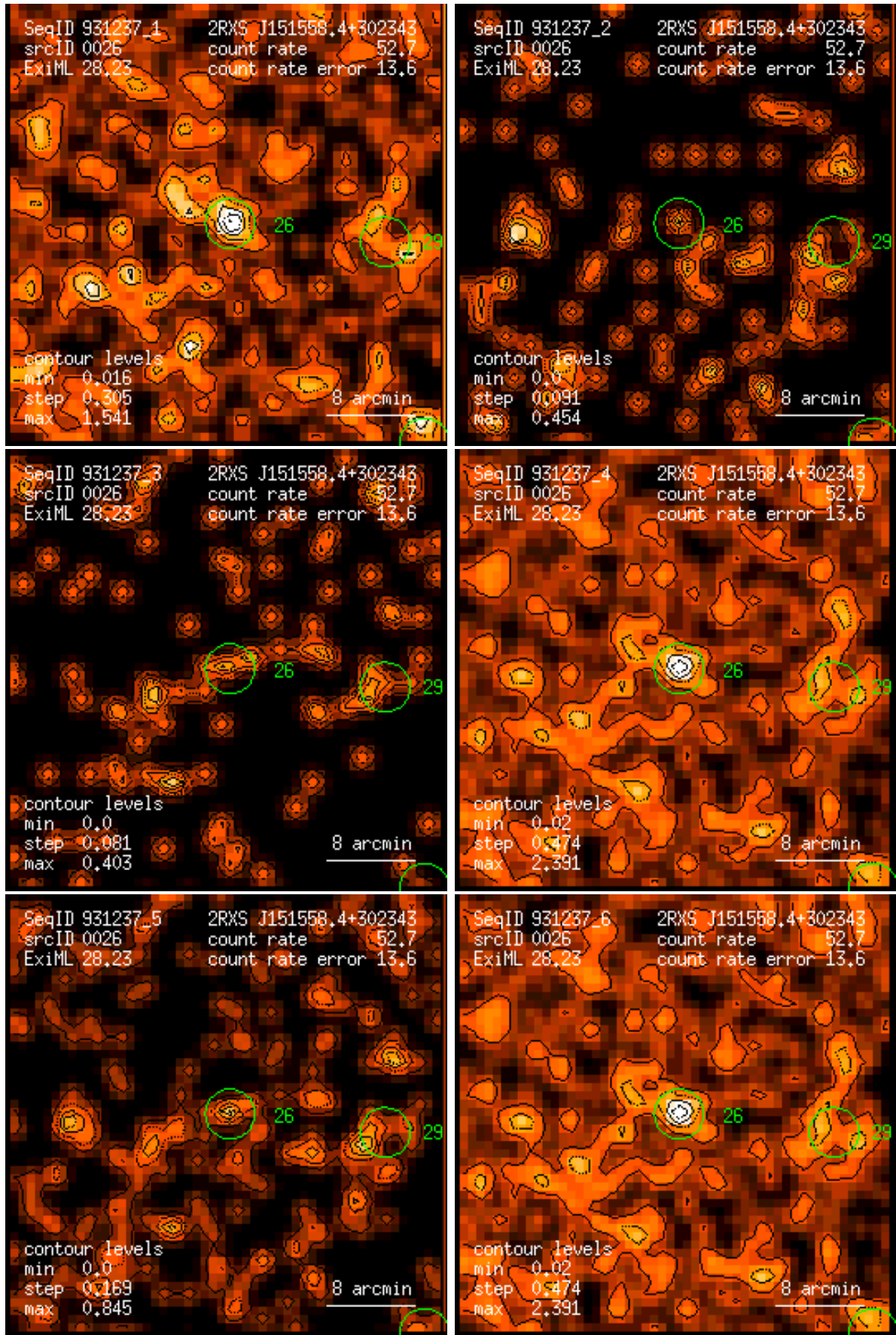
Figure 26: RASS 931237: detection 0026: band rate images, Gaussian filter: (1) PSPC channels 11 – 41, (2) 52 – 90, (3) 91 – 201, (4) 11 – 235, (5) 52 – 201, (6) 11 – 201. Broad band rates in counts/ks. Band rate contour levels in counts/ks/arcmin 2 .
