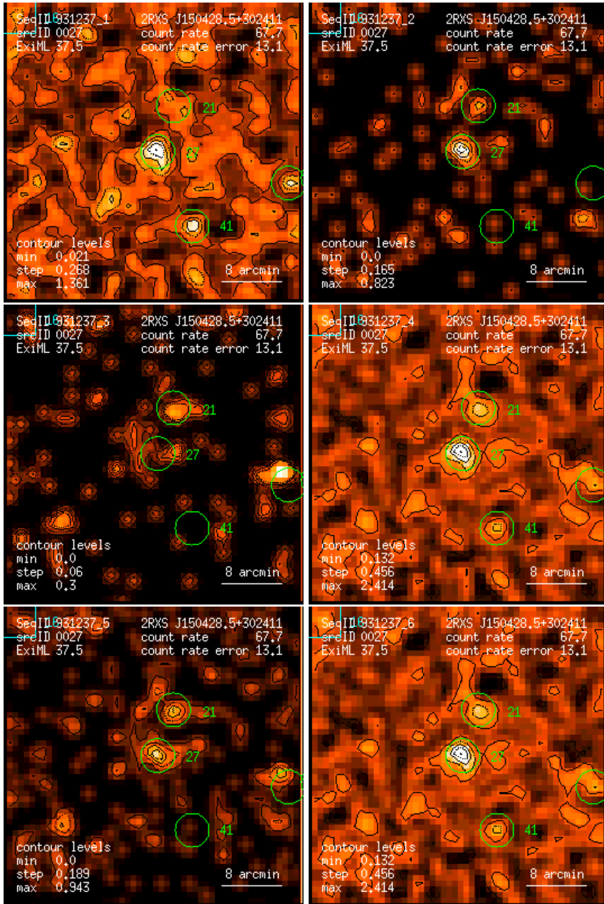
Figure 27: RASS 931237: detection 0027: band rate images, Gaussian filter: (1) PSPC channels 11 – 41, (2) 52 – 90, (3) 91 – 201, (4) 11 – 235, (5) 52 – 201, (6) 11 – 201. Broad band rates in counts/ks. Band rate contour levels in counts/ks/arcmin 2 .
