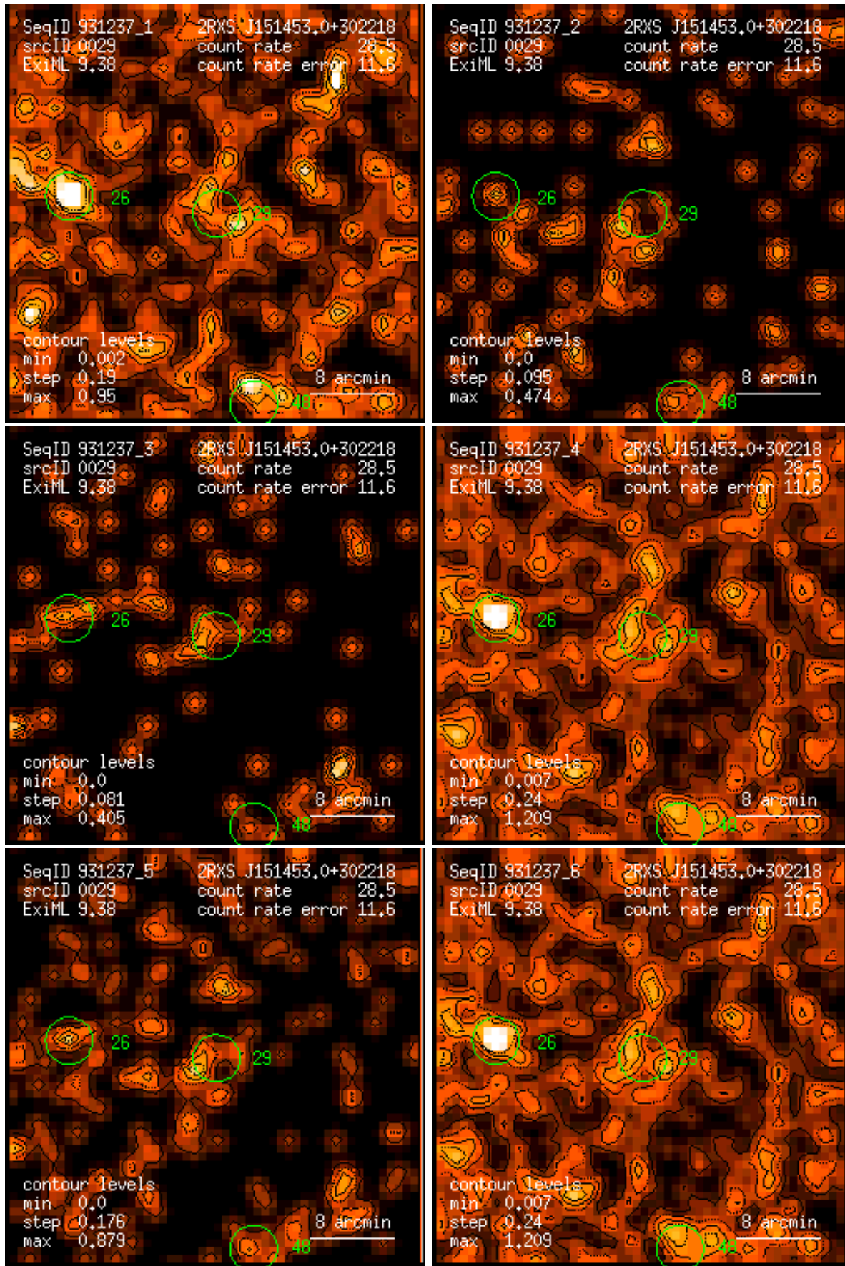
Figure 29: RASS 931237: detection 0029: band rate images, Gaussian filter: (1) PSPC channels 11 – 41, (2) 52 – 90, (3) 91 – 201, (4) 11 – 235, (5) 52 – 201, (6) 11 – 201. Broad band rates in counts/ks. Band rate contour levels in counts/ks/arcmin 2 .
