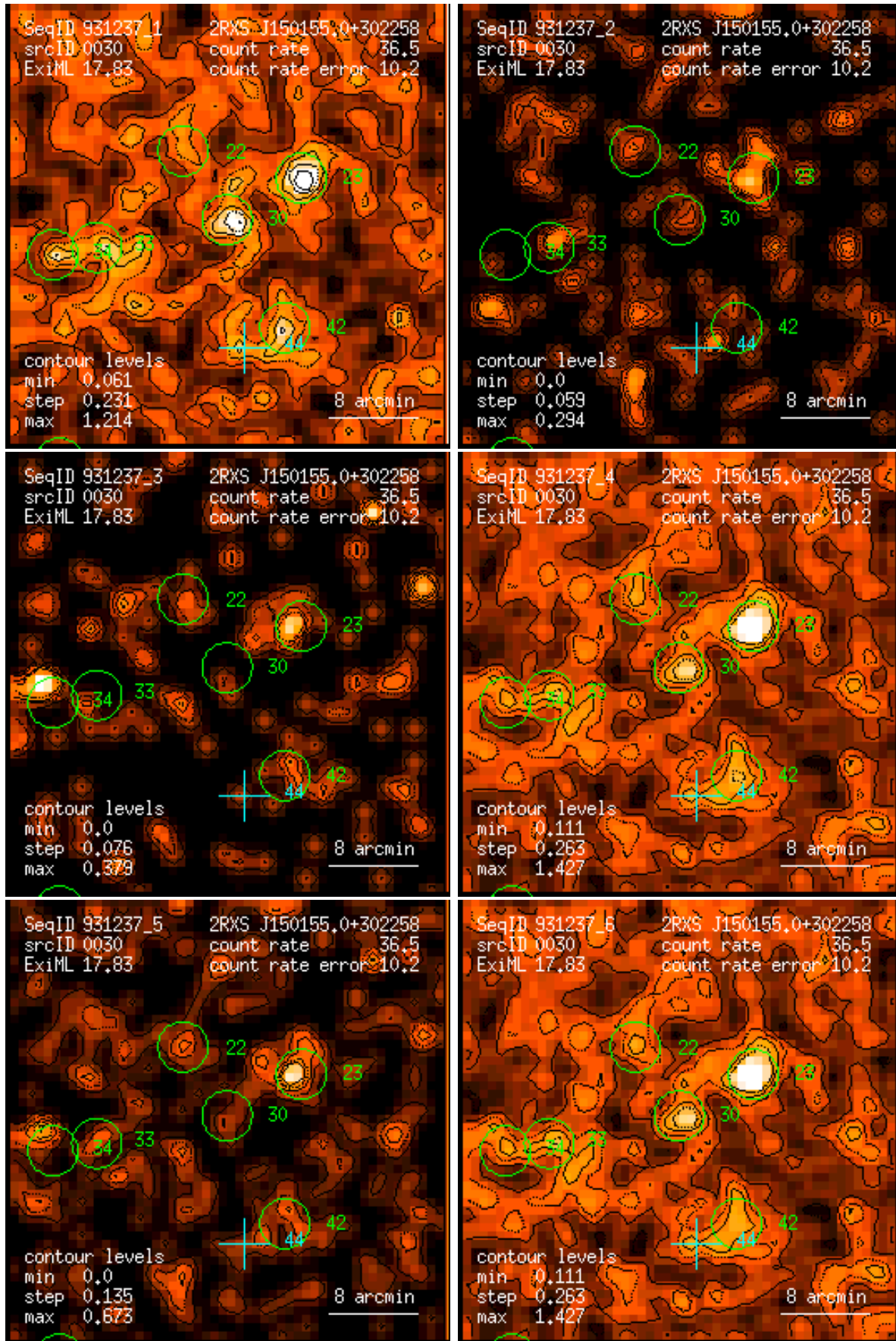
Figure 30: RASS 931237: detection 0030: band rate images, Gaussian filter: (1) PSPC channels 11 – 41, (2) 52 – 90, (3) 91 – 201, (4) 11 – 235, (5) 52 – 201, (6) 11 – 201. Broad band rates in counts/ks. Band rate contour levels in counts/ks/arcmin 2 .
