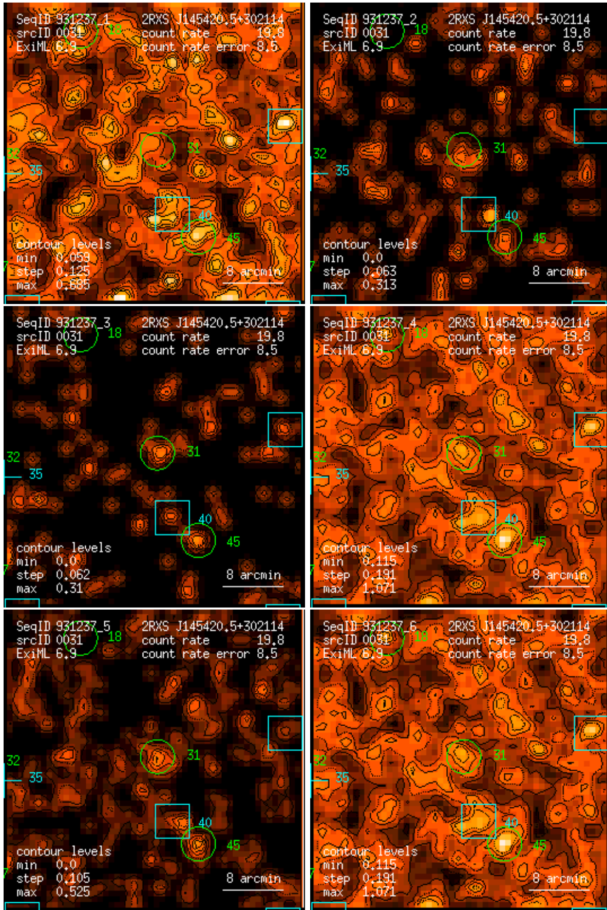
Figure 31: RASS 931237: detection 0031: band rate images, Gaussian filter: (1) PSPC channels 11 – 41, (2) 52 – 90, (3) 91 – 201, (4) 11 – 235, (5) 52 – 201, (6) 11 – 201. Broad band rates in counts/ks. Band rate contour levels in counts/ks/arcmin 2 .
