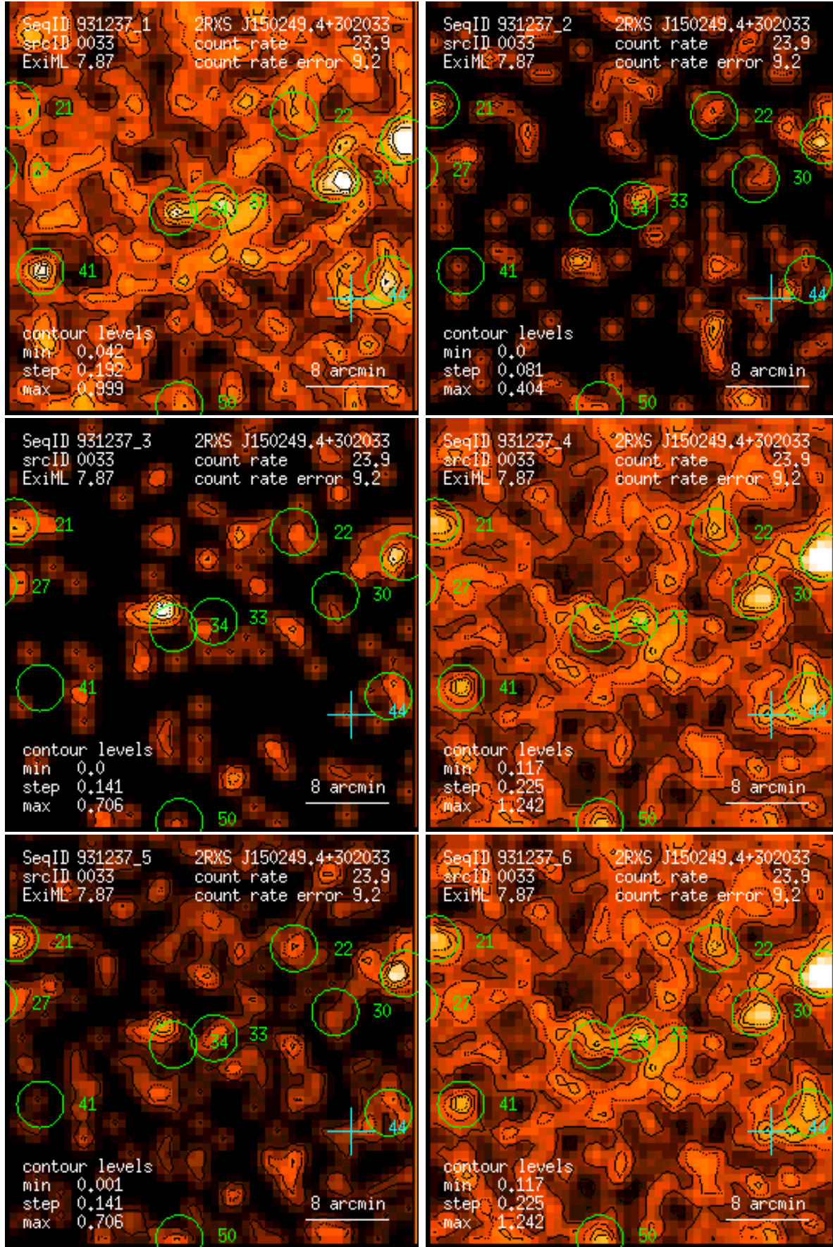
Figure 33: RASS 931237: detection 0033: band rate images, Gaussian filter: (1) PSPC channels 11 – 41, (2) 52 – 90, (3) 91 – 201, (4) 11 – 235, (5) 52 – 201, (6) 11 – 201. Broad band rates in counts/ks. Band rate contour levels in counts/ks/arcmin 2 .
