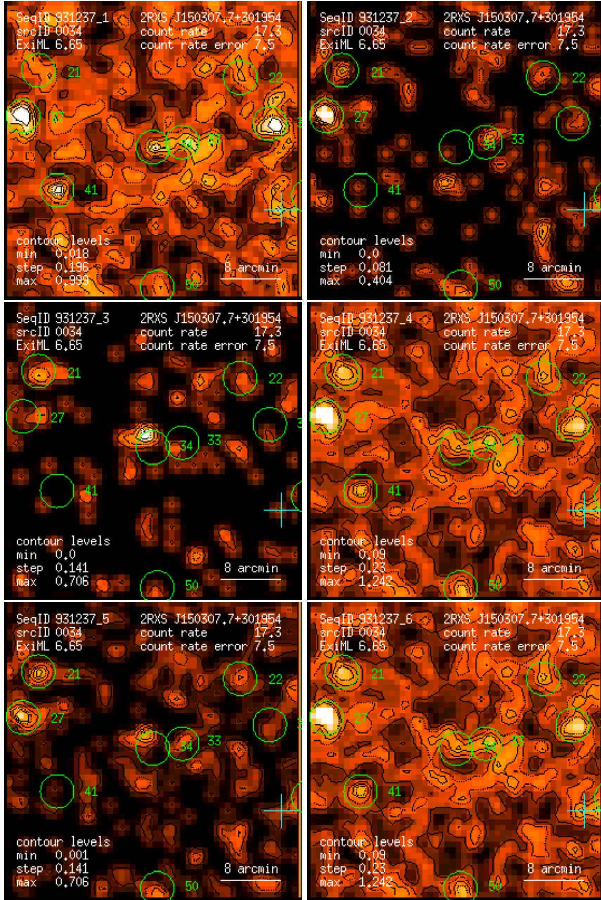
Figure 34: RASS 931237: detection 0034: band rate images, Gaussian filter: (1) PSPC channels 11 – 41, (2) 52 – 90, (3) 91 – 201, (4) 11 – 235, (5) 52 – 201, (6) 11 – 201. Broad band rates in counts/ks. Band rate contour levels in counts/ks/arcmin 2 .
