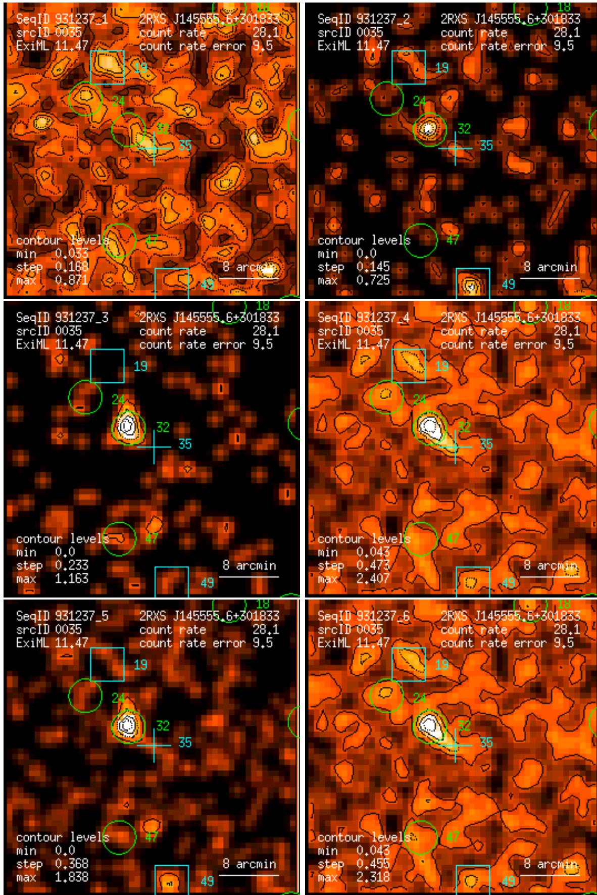
Figure 35: RASS 931237: detection 0035: band rate images, Gaussian filter: (1) PSPC channels 11 – 41, (2) 52 – 90, (3) 91 – 201, (4) 11 – 235, (5) 52 – 201, (6) 11 – 201. Broad band rates in counts/ks. Band rate contour levels in counts/ks/arcmin 2 .
