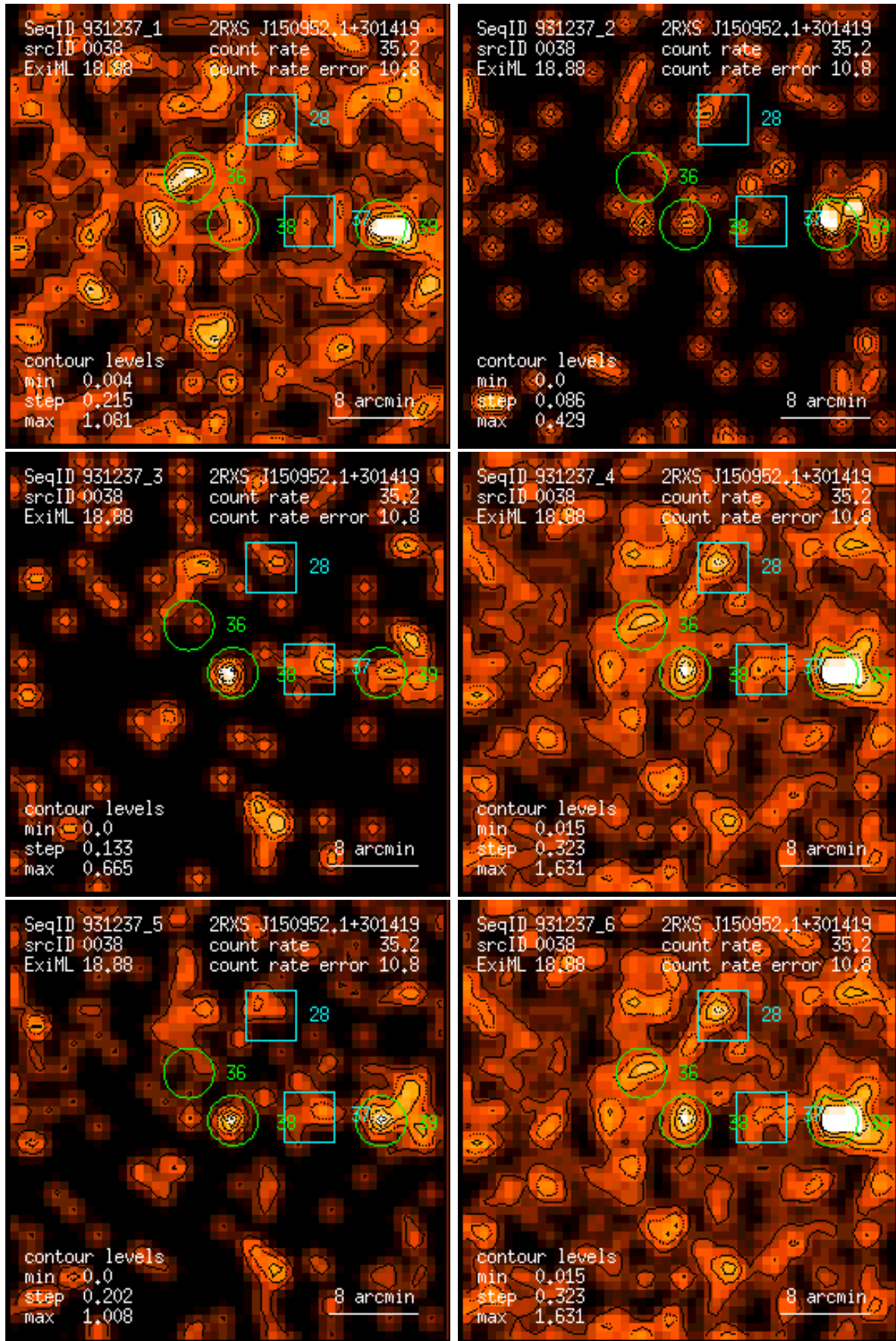
Figure 38: RASS 931237: detection 0038: band rate images, Gaussian filter: (1) PSPC channels 11 – 41, (2) 52 – 90, (3) 91 – 201, (4) 11 – 235, (5) 52 – 201, (6) 11 – 201. Broad band rates in counts/ks. Band rate contour levels in counts/ks/arcmin 2 .
