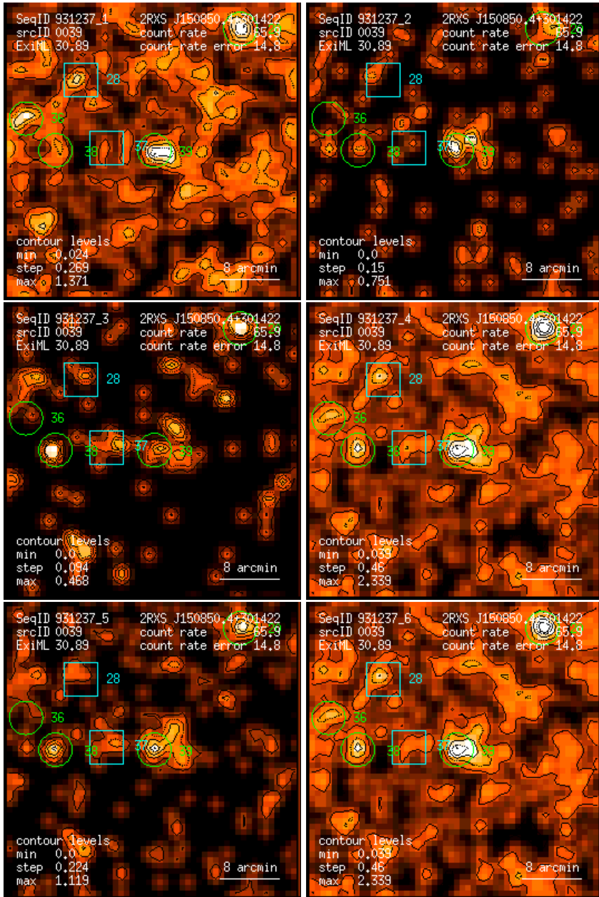
Figure 39: RASS 931237: detection 0039: band rate images, Gaussian filter: (1) PSPC channels 11 – 41, (2) 52 – 90, (3) 91 – 201, (4) 11 – 235, (5) 52 – 201, (6) 11 – 201. Broad band rates in counts/ks. Band rate contour levels in counts/ks/arcmin 2 .
