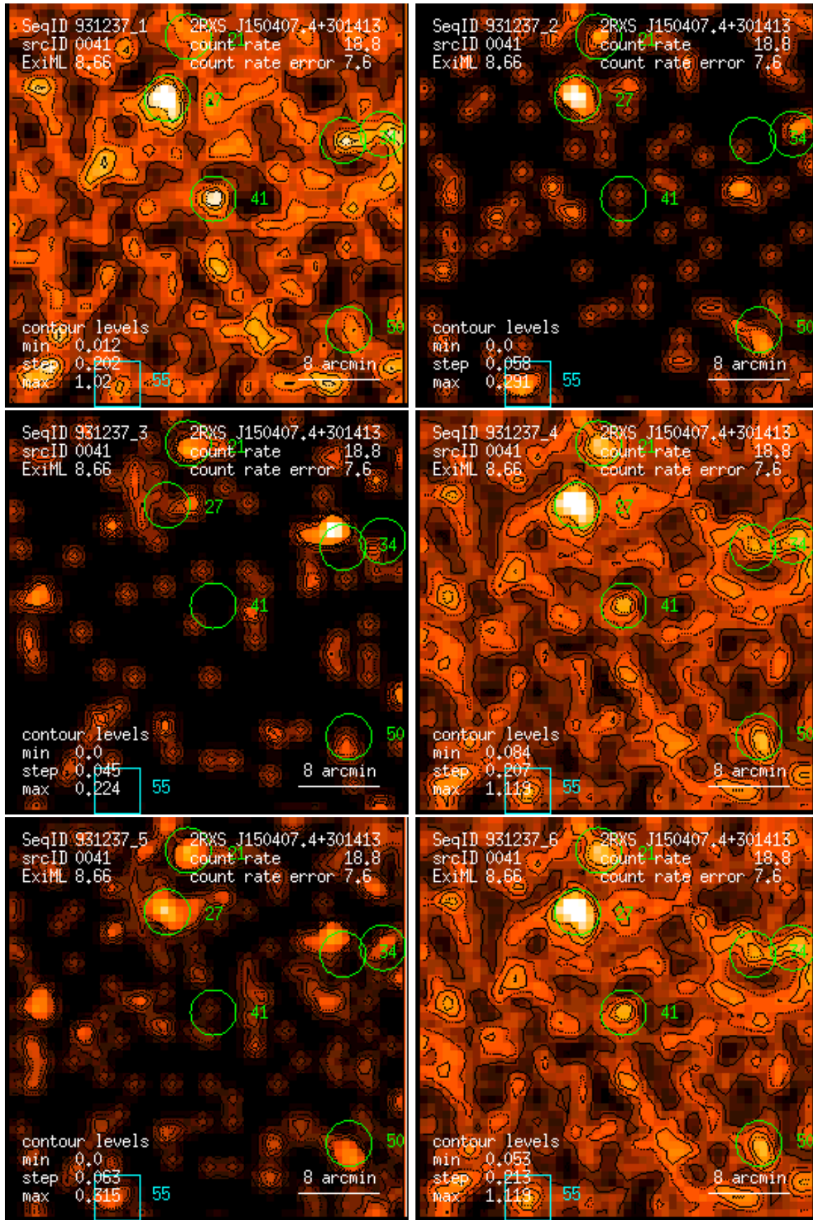
Figure 41: RASS 931237: detection 0041: band rate images, Gaussian filter: (1) PSPC channels 11 – 41, (2) 52 – 90, (3) 91 – 201, (4) 11 – 235, (5) 52 – 201, (6) 11 – 201. Broad band rates in counts/ks. Band rate contour levels in counts/ks/arcmin 2 .
