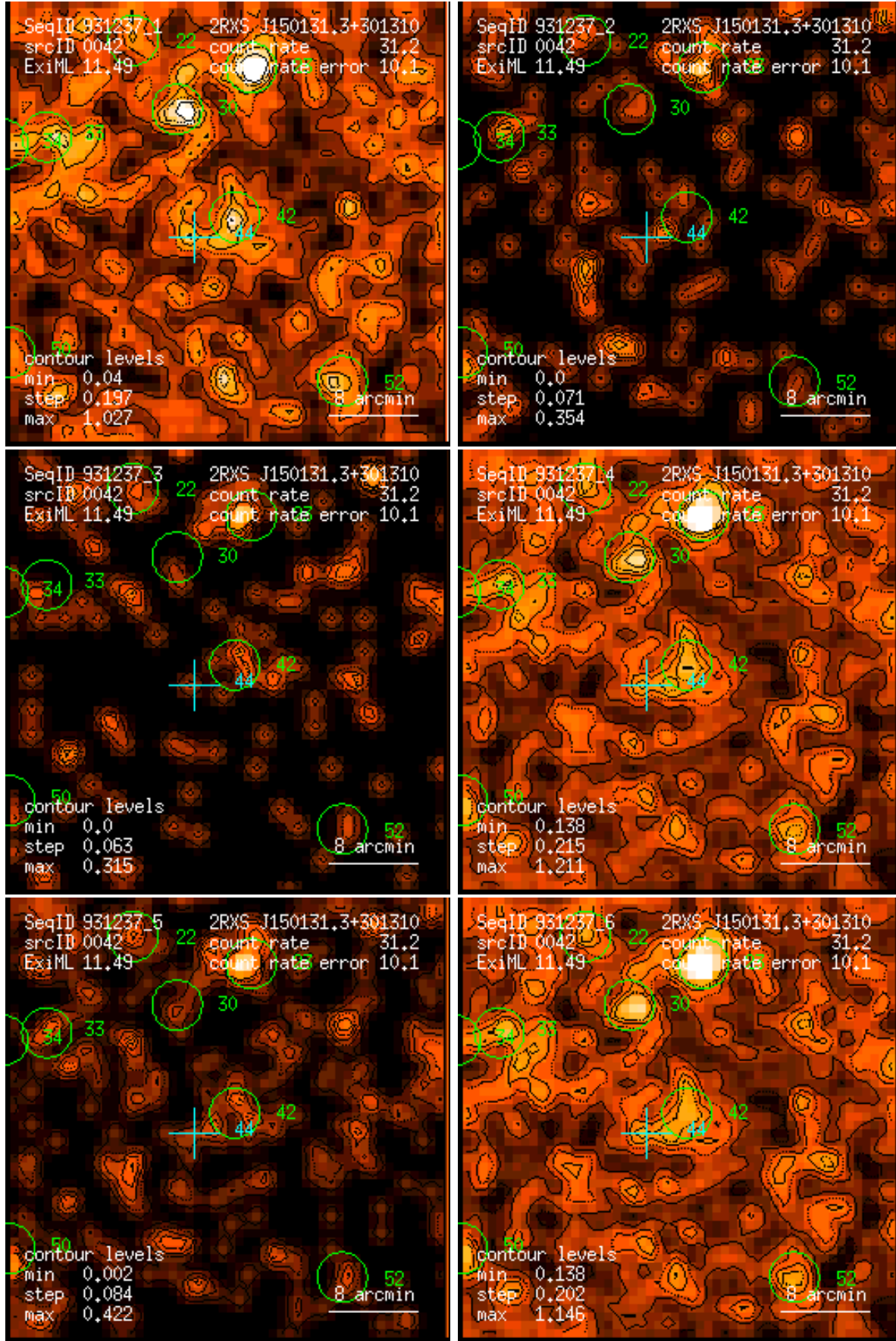
Figure 42: RASS 931237: detection 0042: band rate images, Gaussian filter: (1) PSPC channels 11 – 41, (2) 52 – 90, (3) 91 – 201, (4) 11 – 235, (5) 52 – 201, (6) 11 – 201. Broad band rates in counts/ks. Band rate contour levels in counts/ks/arcmin 2 .
