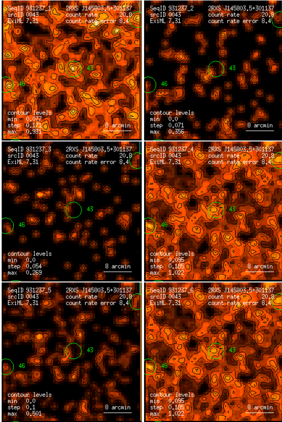
Figure 43: RASS 931237: detection 0043: band rate images, Gaussian filter: (1) PSPC channels 11 – 41, (2) 52 – 90, (3) 91 – 201, (4) 11 – 235, (5) 52 – 201, (6) 11 – 201. Broad band rates in counts/ks. Band rate contour levels in counts/ks/arcmin 2 .
