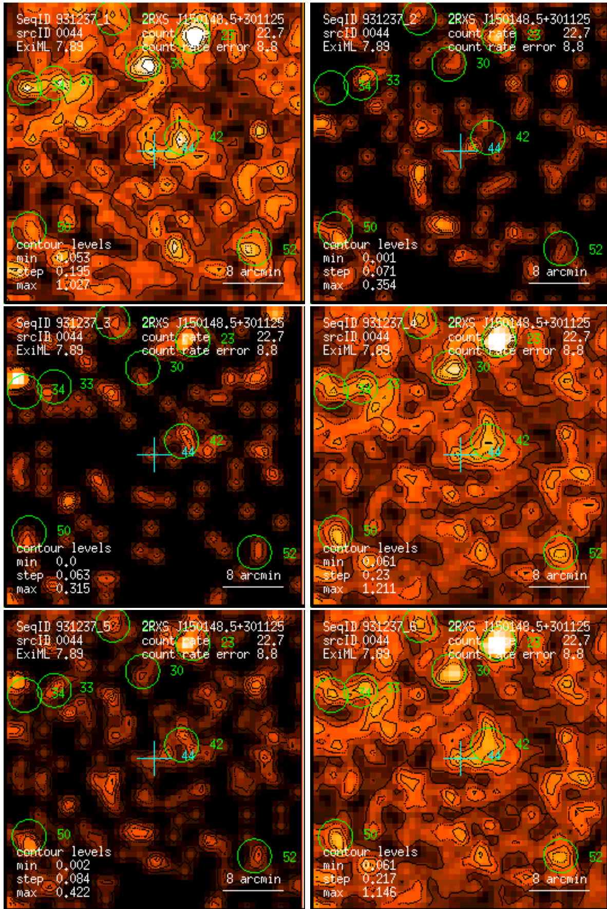
Figure 44: RASS 931237: detection 0044: band rate images, Gaussian filter: (1) PSPC channels 11 – 41, (2) 52 – 90, (3) 91 – 201, (4) 11 – 235, (5) 52 – 201, (6) 11 – 201. Broad band rates in counts/ks. Band rate contour levels in counts/ks/arcmin 2 .
