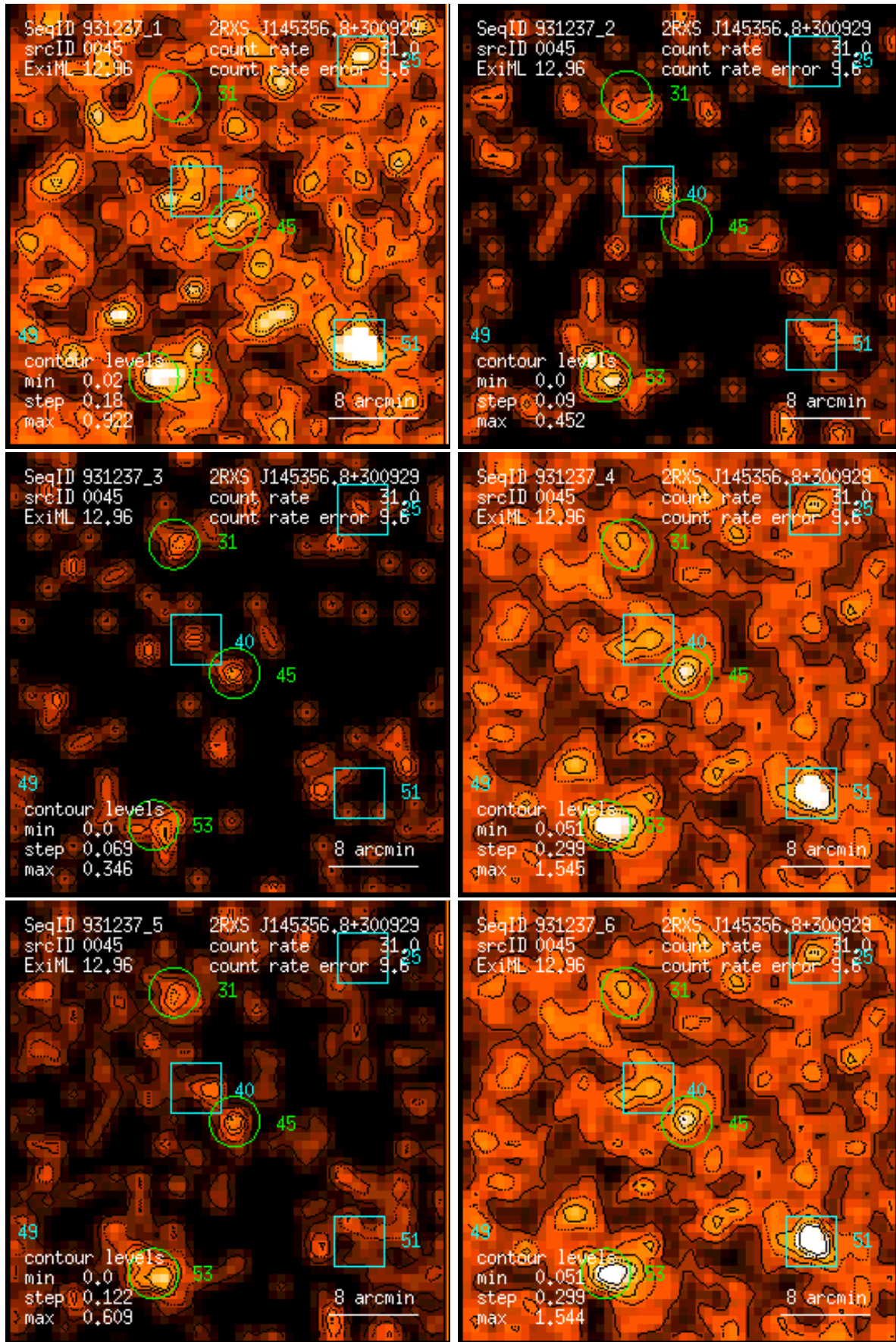
Figure 45: RASS 931237: detection 0045: band rate images, Gaussian filter: (1) PSPC channels 11 – 41, (2) 52 – 90, (3) 91 – 201, (4) 11 – 235, (5) 52 – 201, (6) 11 – 201. Broad band rates in counts/ks. Band rate contour levels in counts/ks/arcmin 2 .
