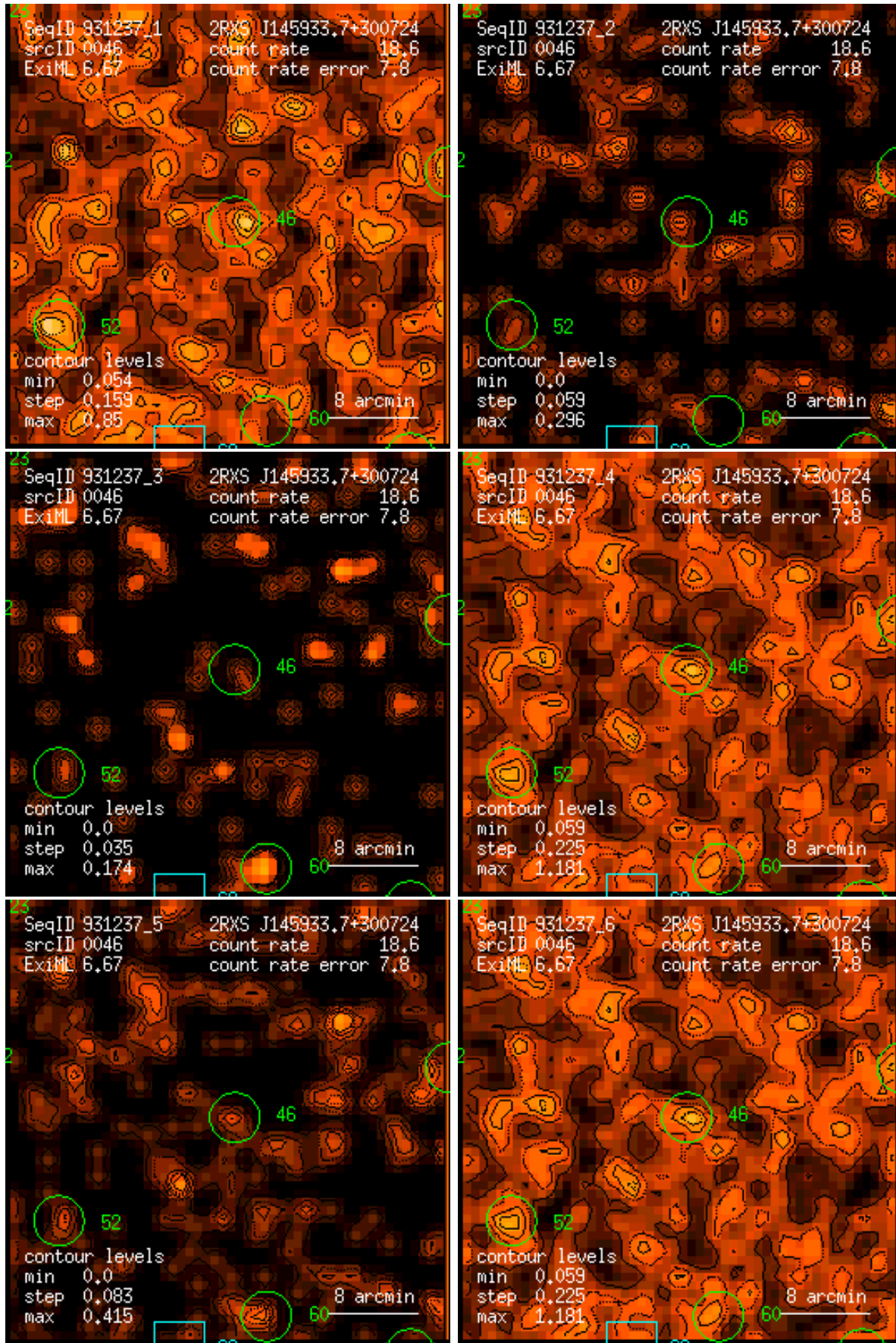
Figure 46: RASS 931237: detection 0046: band rate images, Gaussian filter: (1) PSPC channels 11 – 41, (2) 52 – 90, (3) 91 – 201, (4) 11 – 235, (5) 52 – 201, (6) 11 – 201. Broad band rates in counts/ks. Band rate contour levels in counts/ks/arcmin 2 .
