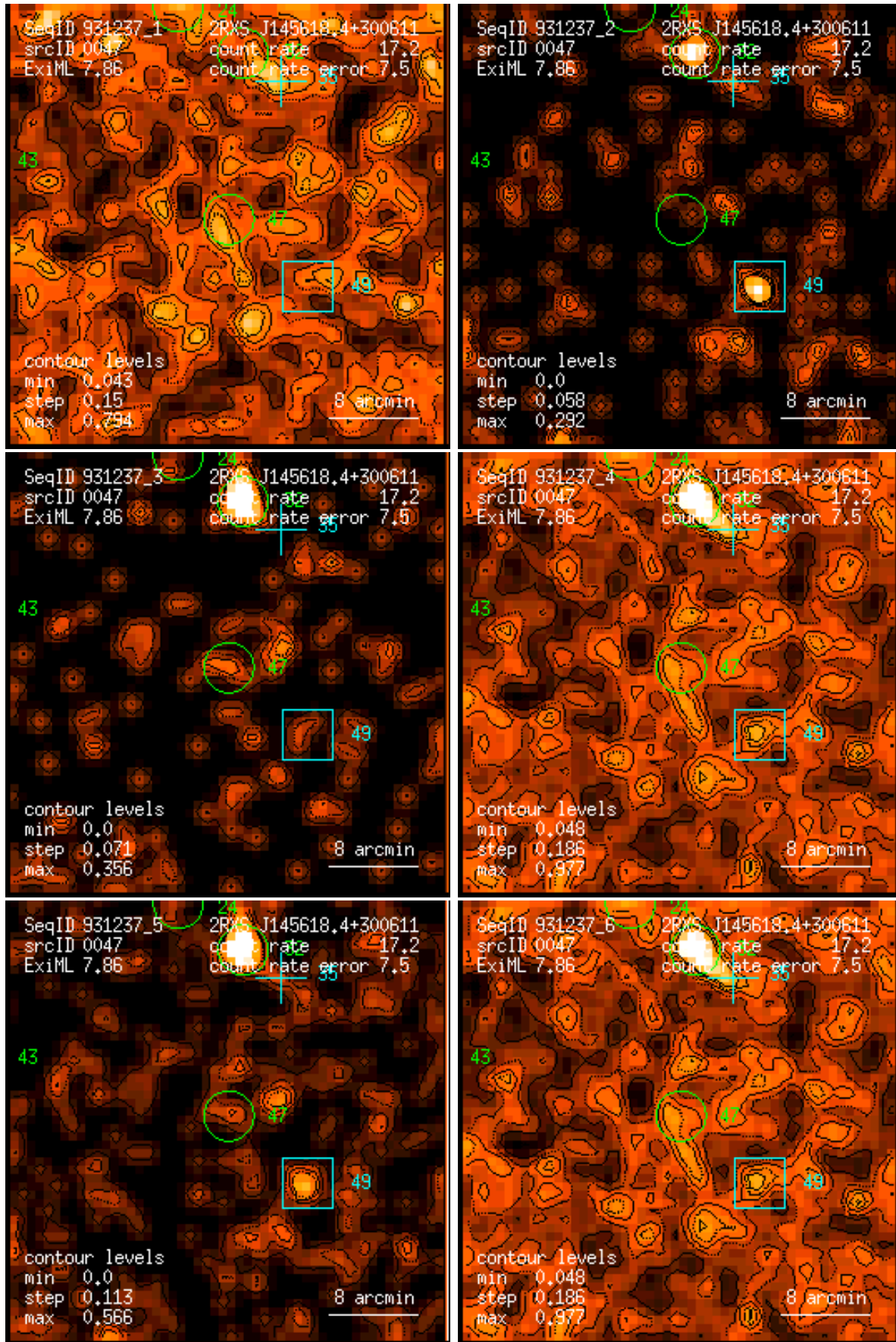
Figure 47: RASS 931237: detection 0047: band rate images, Gaussian filter: (1) PSPC channels 11 – 41, (2) 52 – 90, (3) 91 – 201, (4) 11 – 235, (5) 52 – 201, (6) 11 – 201. Broad band rates in counts/ks. Band rate contour levels in counts/ks/arcmin 2 .
