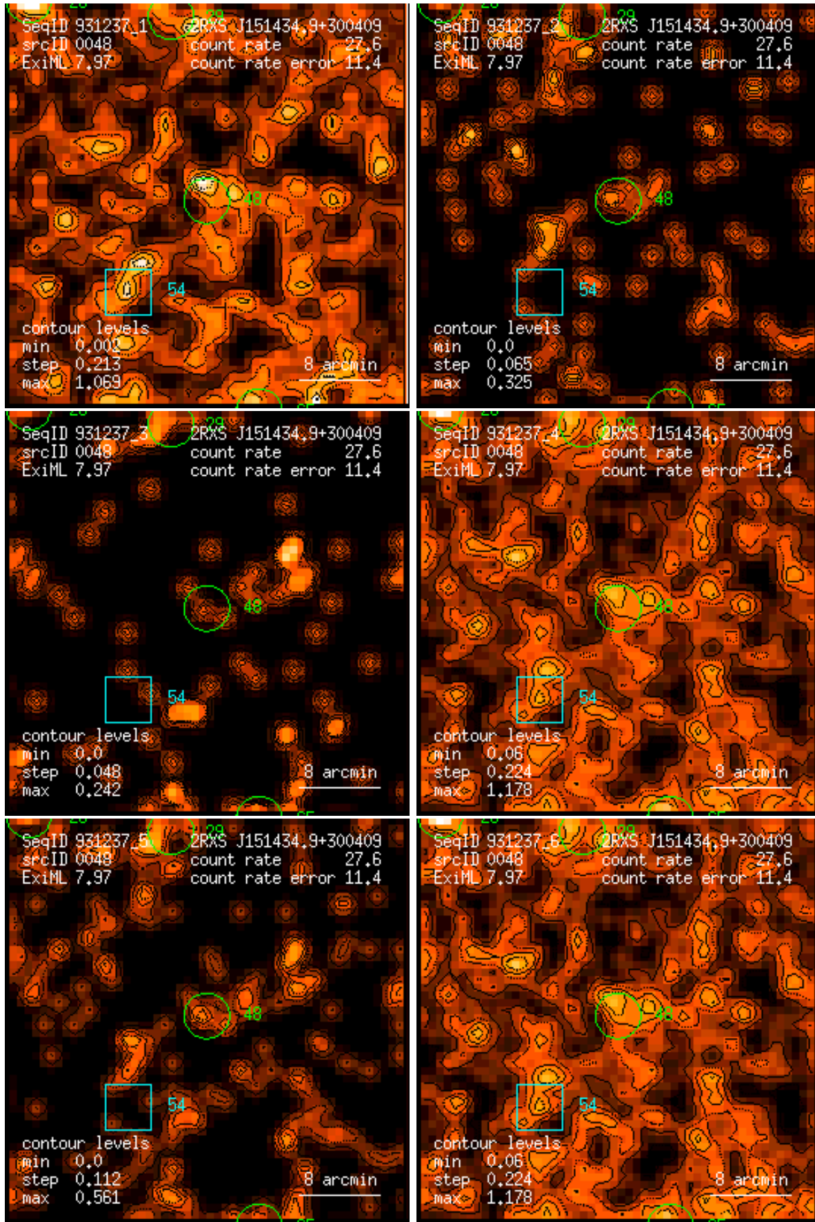
Figure 48: RASS 931237: detection 0048: band rate images, Gaussian filter: (1) PSPC channels 11 – 41, (2) 52 – 90, (3) 91 – 201, (4) 11 – 235, (5) 52 – 201, (6) 11 – 201. Broad band rates in counts/ks. Band rate contour levels in counts/ks/arcmin 2 .
