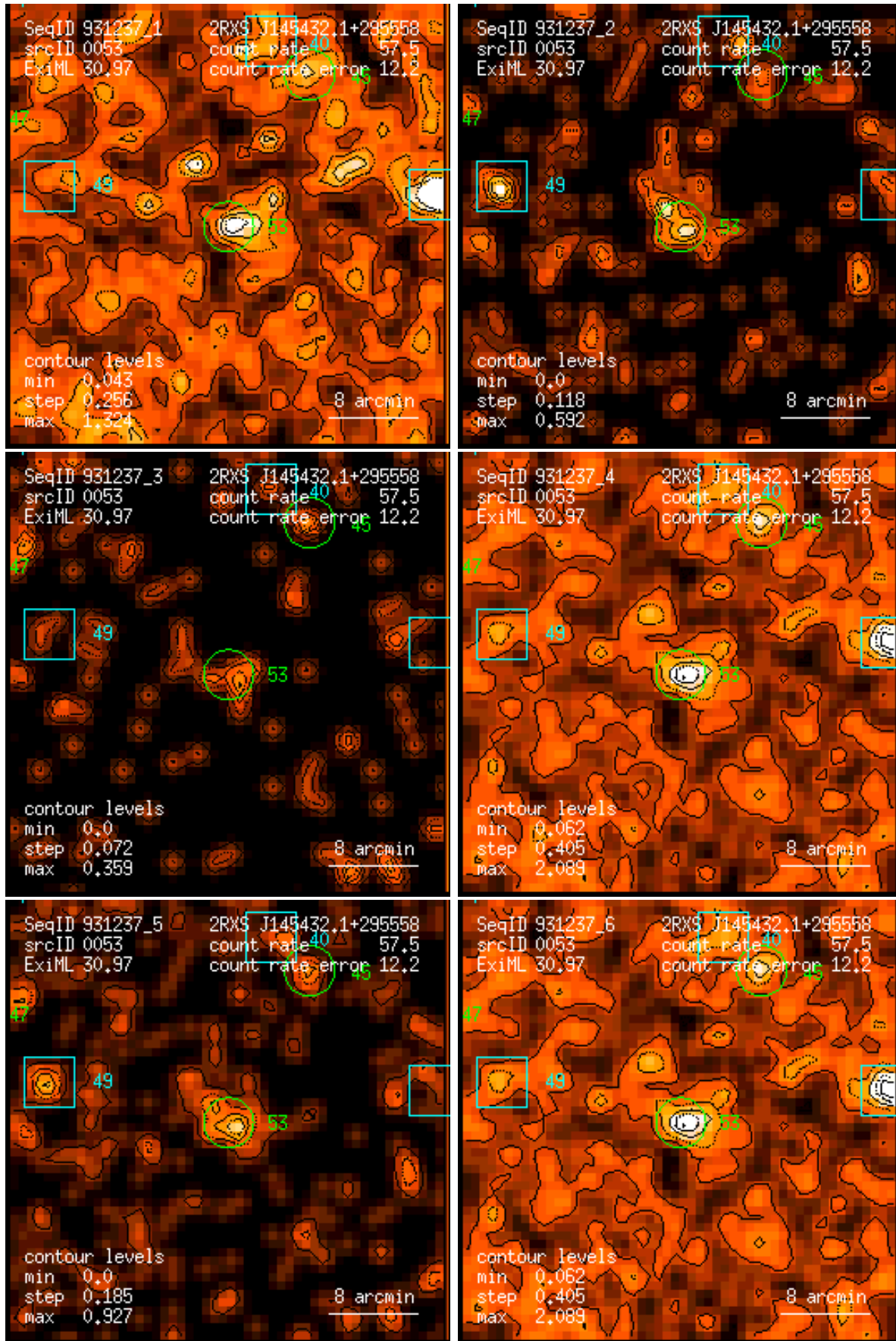
Figure 53: RASS 931237: detection 0053: band rate images, Gaussian filter: (1) PSPC channels 11 – 41, (2) 52 – 90, (3) 91 – 201, (4) 11 – 235, (5) 52 – 201, (6) 11 – 201. Broad band rates in counts/ks. Band rate contour levels in counts/ks/arcmin 2 .
