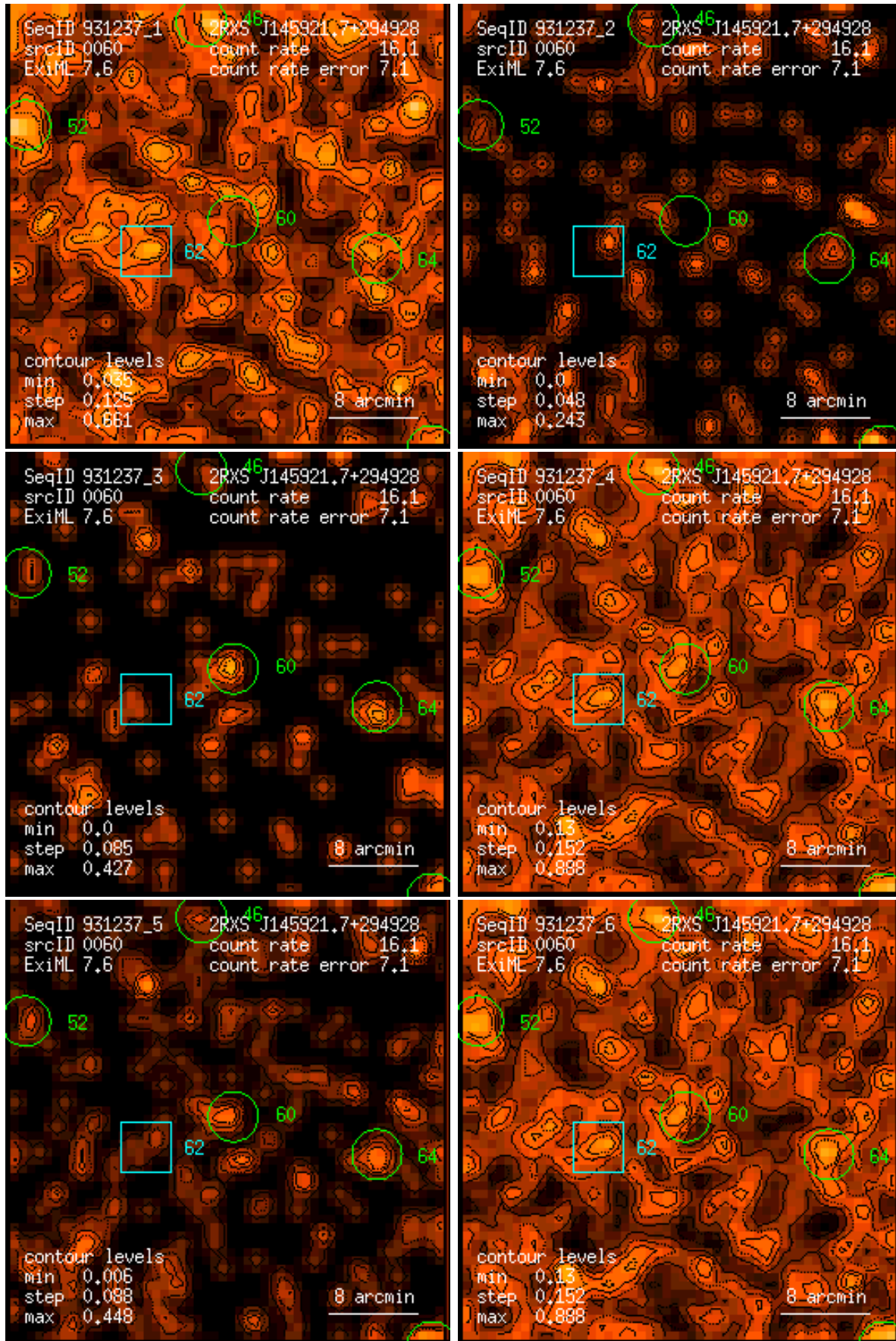
Figure 60: RASS 931237: detection 0060: band rate images, Gaussian filter: (1) PSPC channels 11 – 41, (2) 52 – 90, (3) 91 – 201, (4) 11 – 235, (5) 52 – 201, (6) 11 – 201. Broad band rates in counts/ks. Band rate contour levels in counts/ks/arcmin 2 .
