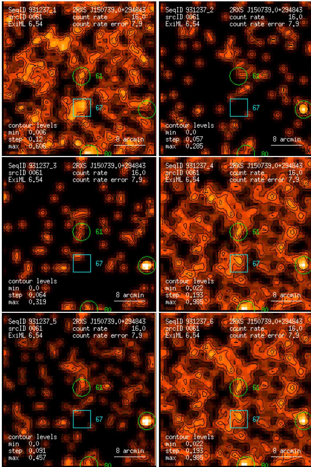
Figure 61: RASS 931237: detection 0061: band rate images, Gaussian filter: (1) PSPC channels 11 – 41, (2) 52 – 90, (3) 91 – 201, (4) 11 – 235, (5) 52 – 201, (6) 11 – 201. Broad band rates in counts/ks. Band rate contour levels in counts/ks/arcmin 2 .
