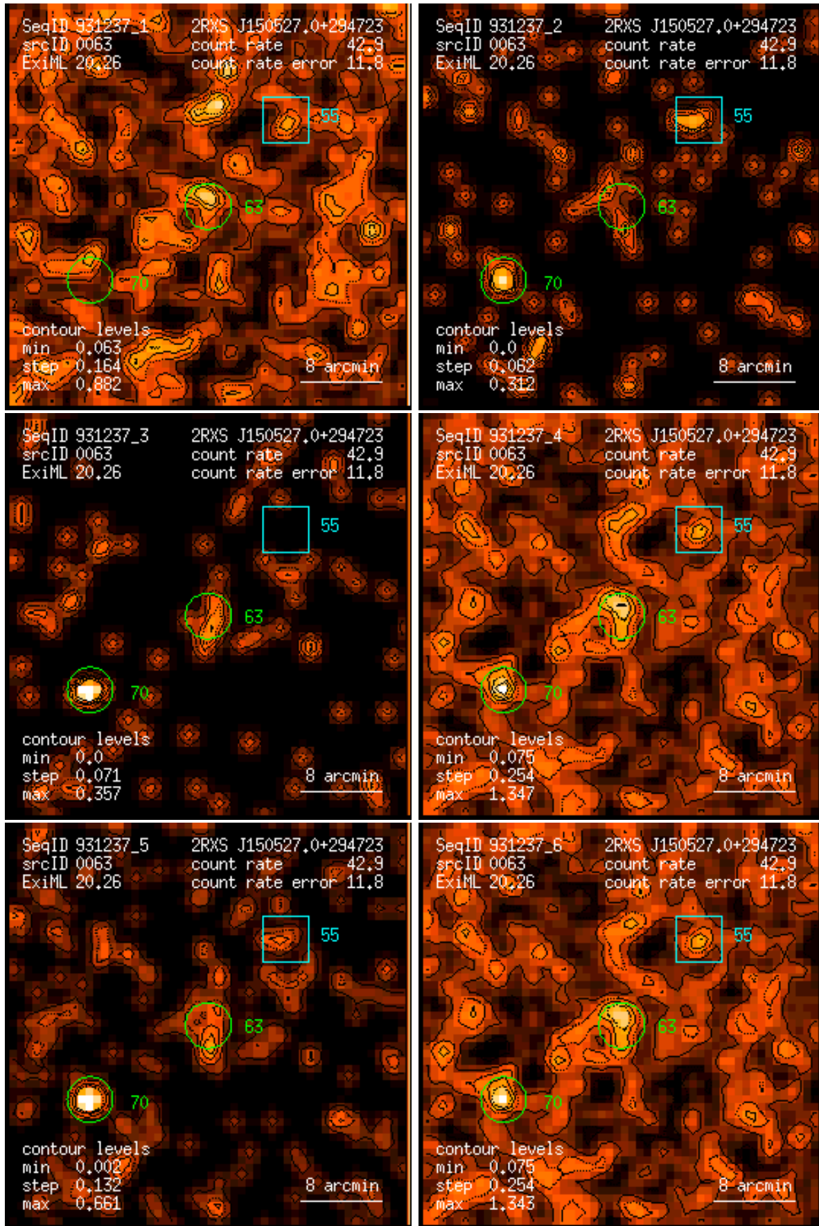
Figure 63: RASS 931237: detection 0063: band rate images, Gaussian filter: (1) PSPC channels 11 – 41, (2) 52 – 90, (3) 91 – 201, (4) 11 – 235, (5) 52 – 201, (6) 11 – 201. Broad band rates in counts/ks. Band rate contour levels in counts/ks/arcmin 2 .
