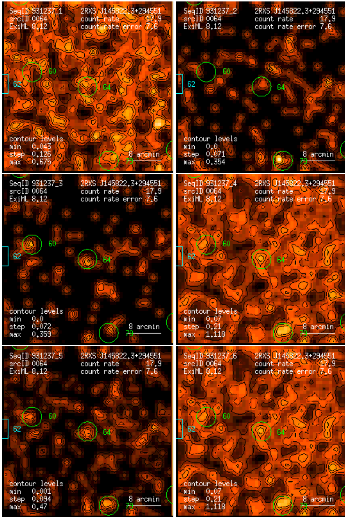
Figure 64: RASS 931237: detection 0064: band rate images, Gaussian filter: (1) PSPC channels 11 – 41, (2) 52 – 90, (3) 91 – 201, (4) 11 – 235, (5) 52 – 201, (6) 11 – 201. Broad band rates in counts/ks. Band rate contour levels in counts/ks/arcmin 2 .
