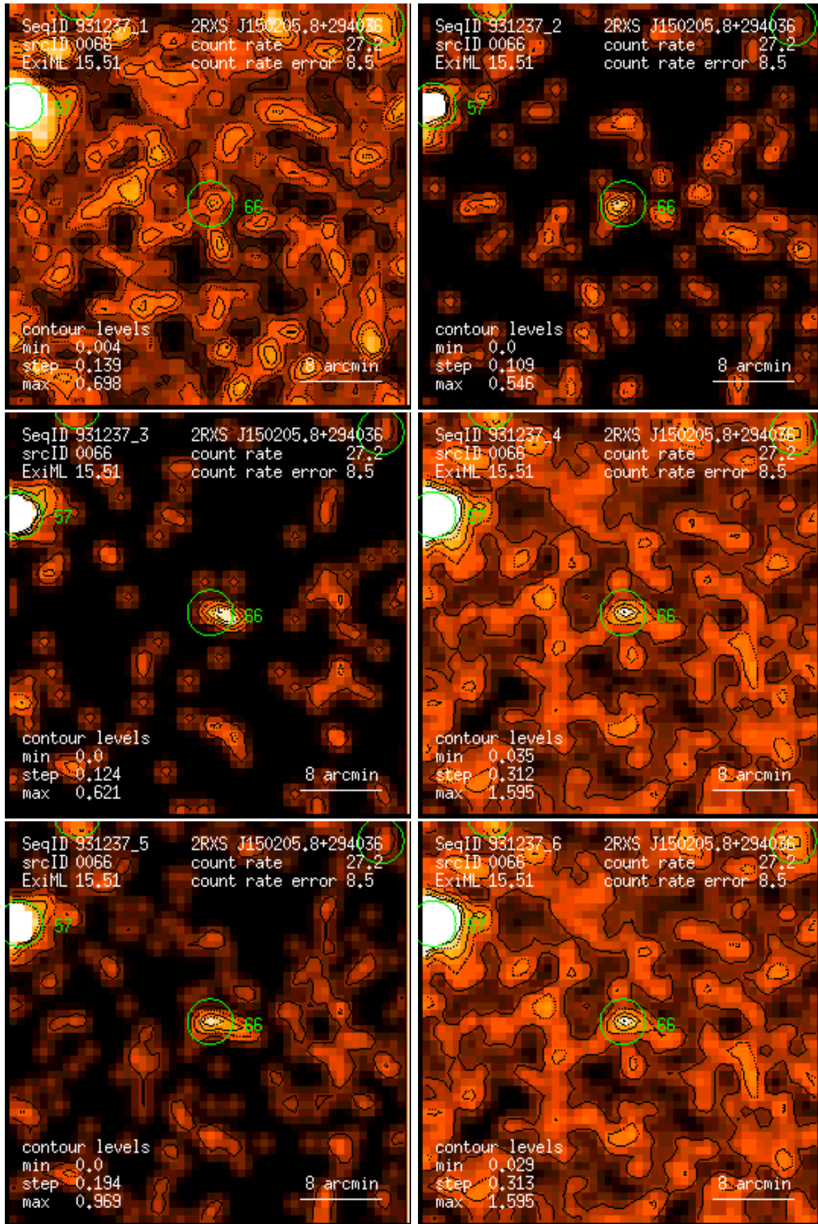
Figure 66: RASS 931237: detection 0066: band rate images, Gaussian filter: (1) PSPC channels 11 – 41, (2) 52 – 90, (3) 91 – 201, (4) 11 – 235, (5) 52 – 201, (6) 11 – 201. Broad band rates in counts/ks. Band rate contour levels in counts/ks/arcmin 2 .
