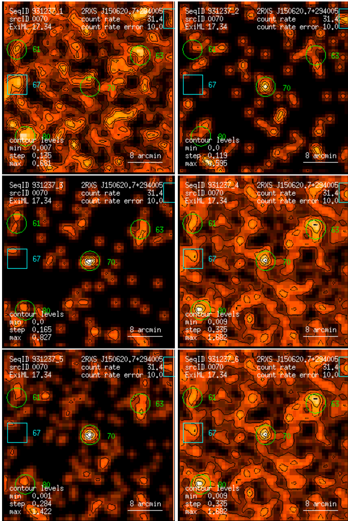
Figure 70: RASS 931237: detection 0070: band rate images, Gaussian filter: (1) PSPC channels 11 – 41, (2) 52 – 90, (3) 91 – 201, (4) 11 – 235, (5) 52 – 201, (6) 11 – 201. Broad band rates in counts/ks. Band rate contour levels in counts/ks/arcmin 2 .
