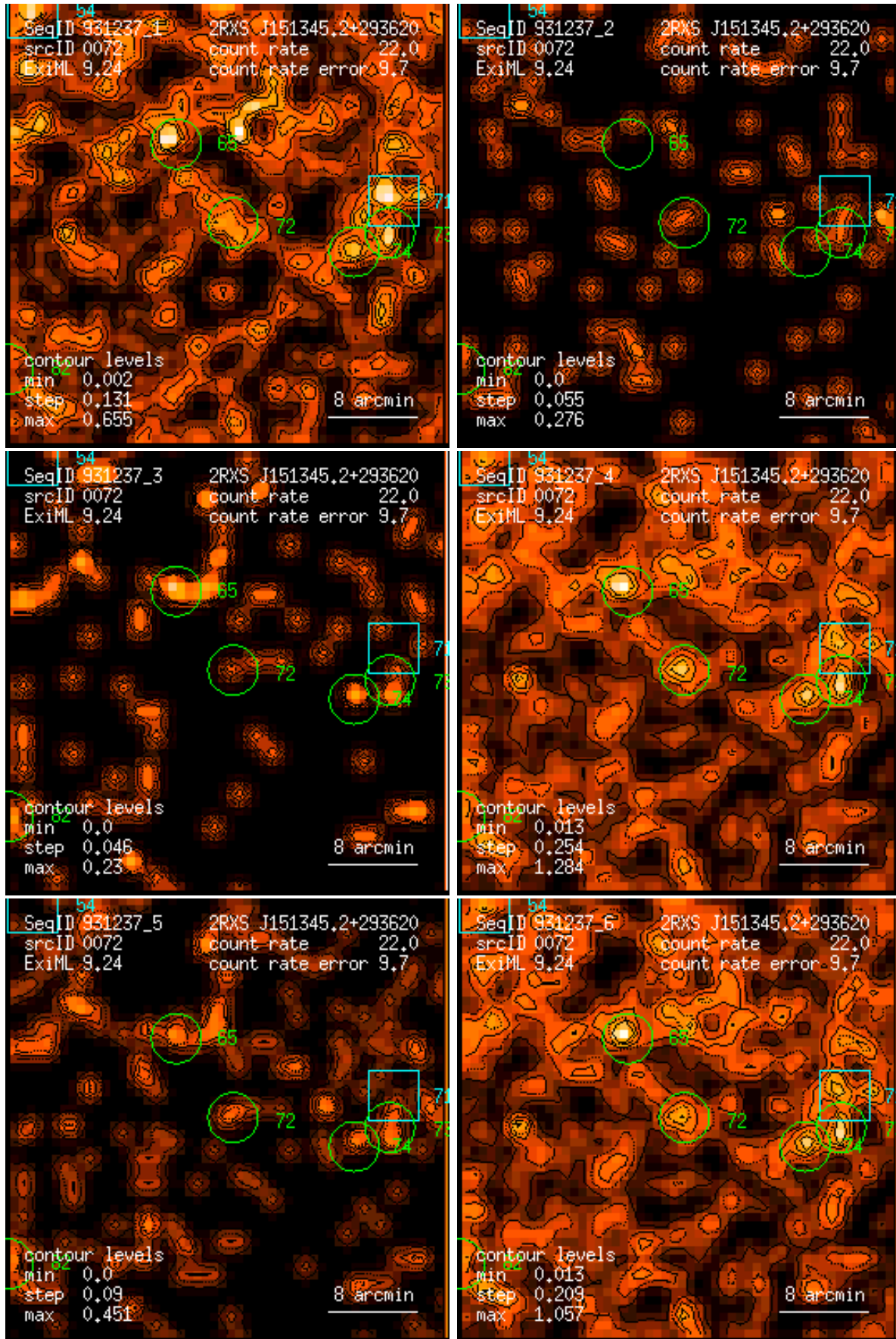
Figure 72: RASS 931237: detection 0072: band rate images, Gaussian filter: (1) PSPC channels 11 – 41, (2) 52 – 90, (3) 91 – 201, (4) 11 – 235, (5) 52 – 201, (6) 11 – 201. Broad band rates in counts/ks. Band rate contour levels in counts/ks/arcmin 2 .
