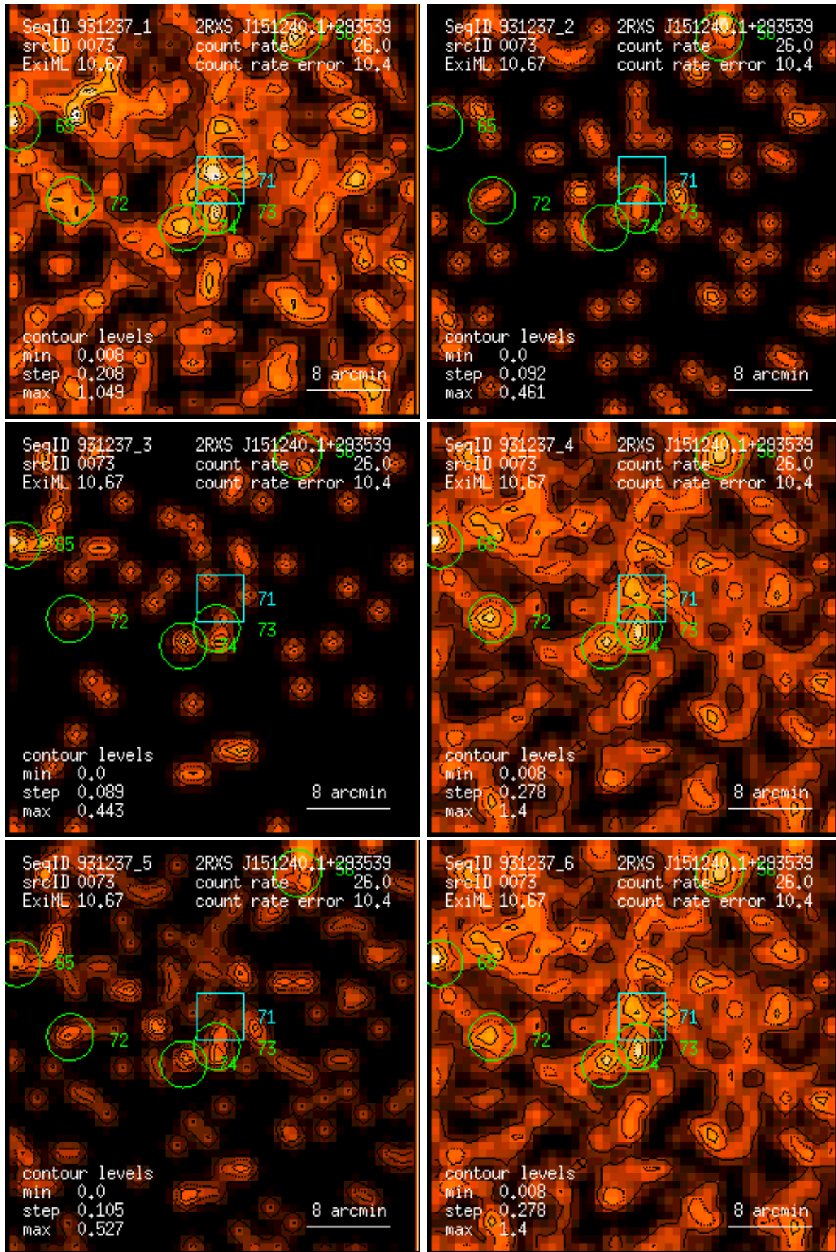
Figure 73: RASS 931237: detection 0073: band rate images, Gaussian filter: (1) PSPC channels 11 – 41, (2) 52 – 90, (3) 91 – 201, (4) 11 – 235, (5) 52 – 201, (6) 11 – 201. Broad band rates in counts/ks. Band rate contour levels in counts/ks/arcmin 2 .
