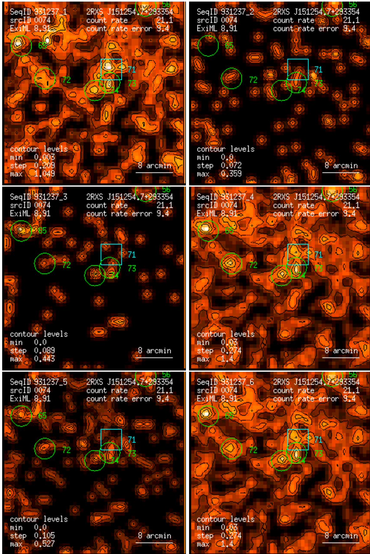
Figure 74: RASS 931237: detection 0074: band rate images, Gaussian filter: (1) PSPC channels 11 – 41, (2) 52 – 90, (3) 91 – 201, (4) 11 – 235, (5) 52 – 201, (6) 11 – 201. Broad band rates in counts/ks. Band rate contour levels in counts/ks/arcmin 2 .
