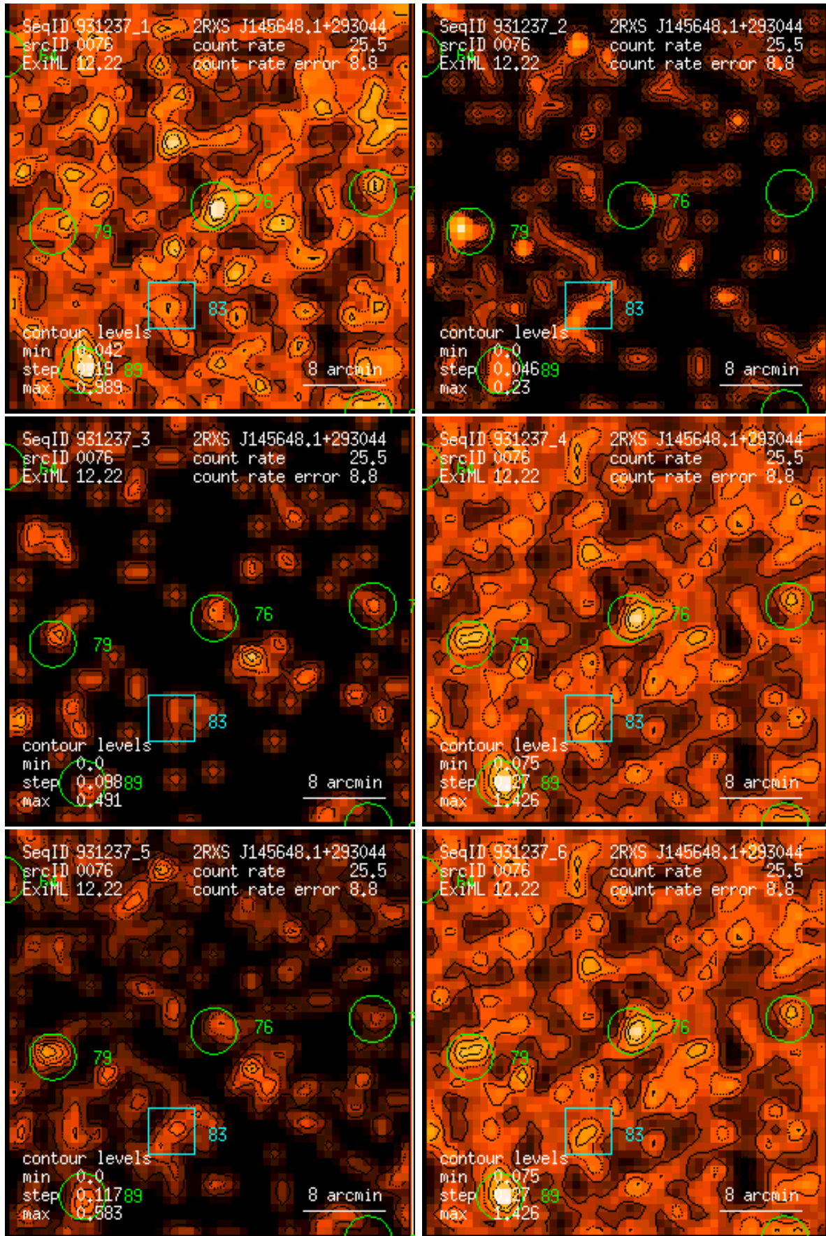
Figure 76: RASS 931237: detection 0076: band rate images, Gaussian filter: (1) PSPC channels 11 – 41, (2) 52 – 90, (3) 91 – 201, (4) 11 – 235, (5) 52 – 201, (6) 11 – 201. Broad band rates in counts/ks. Band rate contour levels in counts/ks/arcmin 2 .
