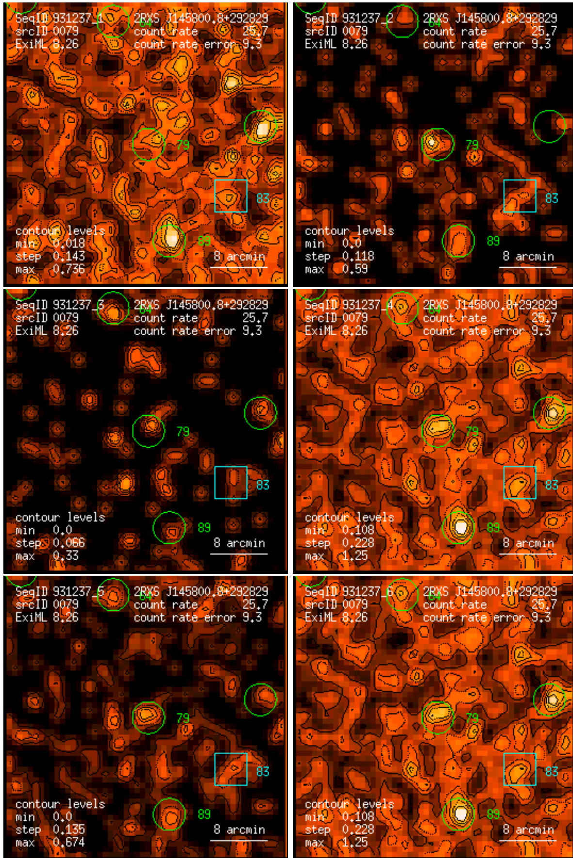
Figure 79: RASS 931237: detection 0079: band rate images, Gaussian filter: (1) PSPC channels 11 – 41, (2) 52 – 90, (3) 91 – 201, (4) 11 – 235, (5) 52 – 201, (6) 11 – 201. Broad band rates in counts/ks. Band rate contour levels in counts/ks/arcmin 2 .
