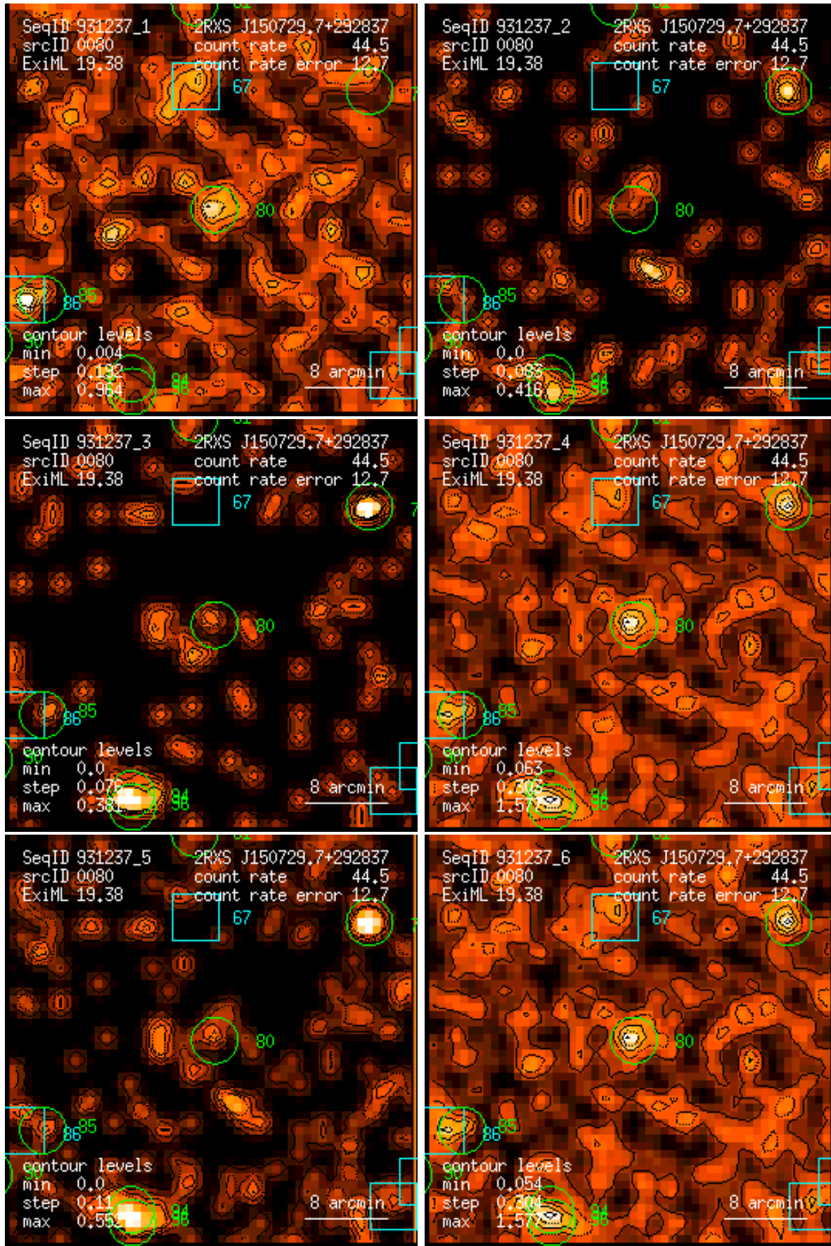
Figure 80: RASS 931237: detection 0080: band rate images, Gaussian filter: (1) PSPC channels 11 – 41, (2) 52 – 90, (3) 91 – 201, (4) 11 – 235, (5) 52 – 201, (6) 11 – 201. Broad band rates in counts/ks. Band rate contour levels in counts/ks/arcmin 2 .
