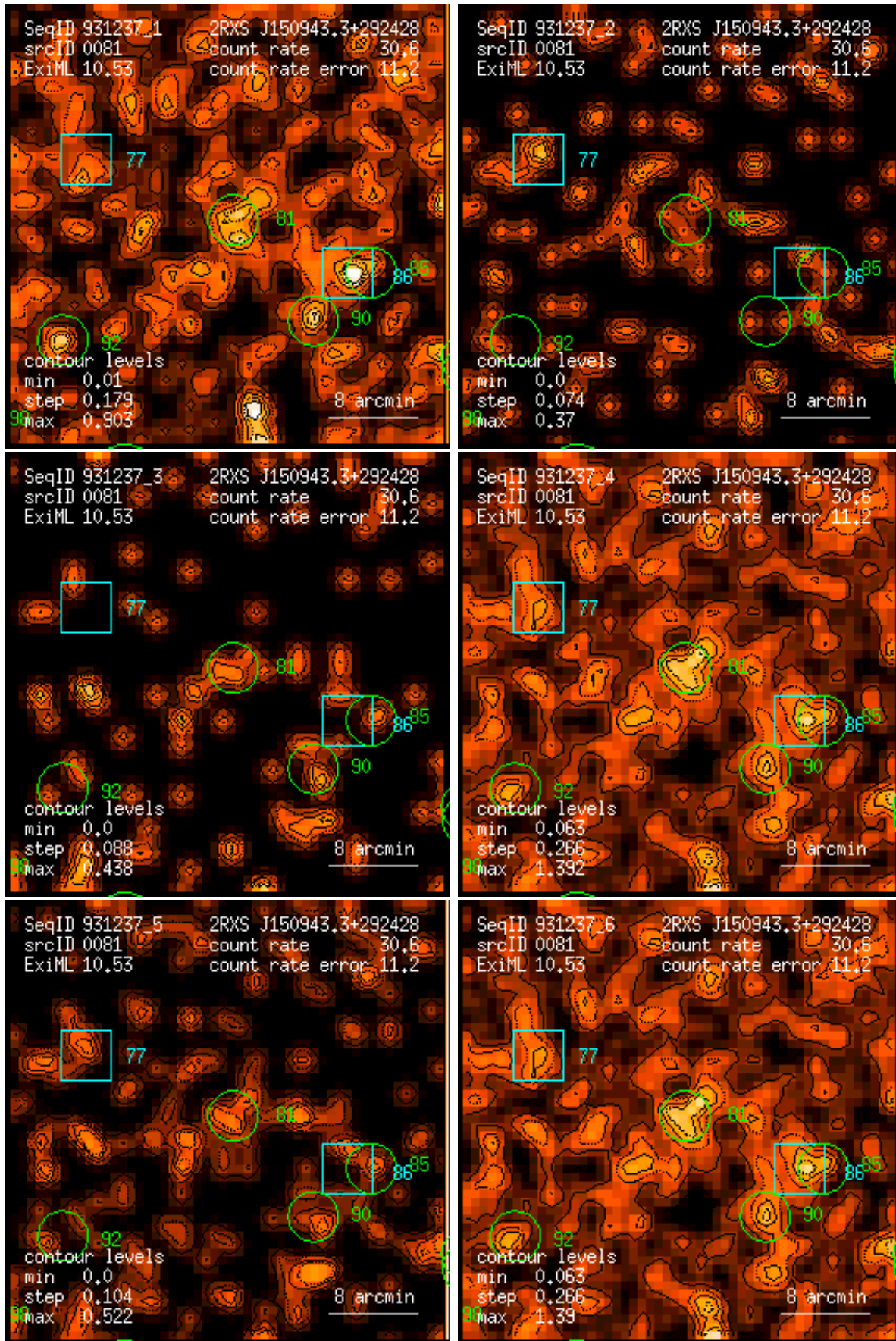
Figure 81: RASS 931237: detection 0081: band rate images, Gaussian filter: (1) PSPC channels 11 – 41, (2) 52 – 90, (3) 91 – 201, (4) 11 – 235, (5) 52 – 201, (6) 11 – 201. Broad band rates in counts/ks. Band rate contour levels in counts/ks/arcmin 2 .
